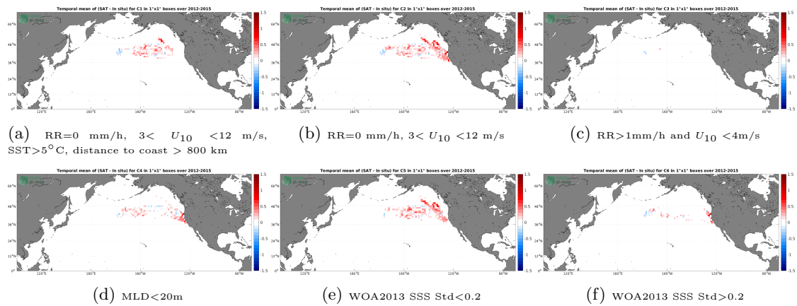
Figure 12: Temporal mean gridded over spatial boxes of size 1^\circ \times 1^\circ of \Delta SSS (Aquarius SSS L3 CAP v5 - Monthly (JPL) - Marine mammals) for 6 different subdatasets corresponding to:RR=0 mm/h, 3 < U_{10} < 12 m/s, SST >5^\circ C, distance to coast > 800 km (a), RR=0 mm/h, 3 < U_{10} < 12 m/s (b), RR >1 mm/h and U_{10} < 4 m/s (c),MLD <20 m (d),WOA2013 SSS Std <0.2 (e),WOA2013 SSS Std >0.2 (f).
