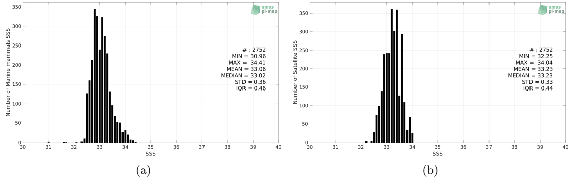
Figure 2: Histograms of SSS from Marine mammals (a) and Aquarius SSS L3 CAP v5 - Monthly (JPL) (b) considering all match-up pairs per bins of 0.1 over the North Pacific Ocean Pi-MEP region and for the full satellite product period.
