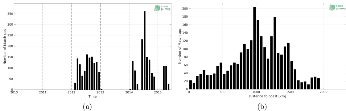
Figure 1: Number of match-ups between Marine mammals and Aquarius SSS L3 CAP v5 - Monthly (JPL) SSS as a function of time (a) and as function of the distance to coast (b) over the North Pacific Ocean Pi-MEP region and for the full satellite product period.
