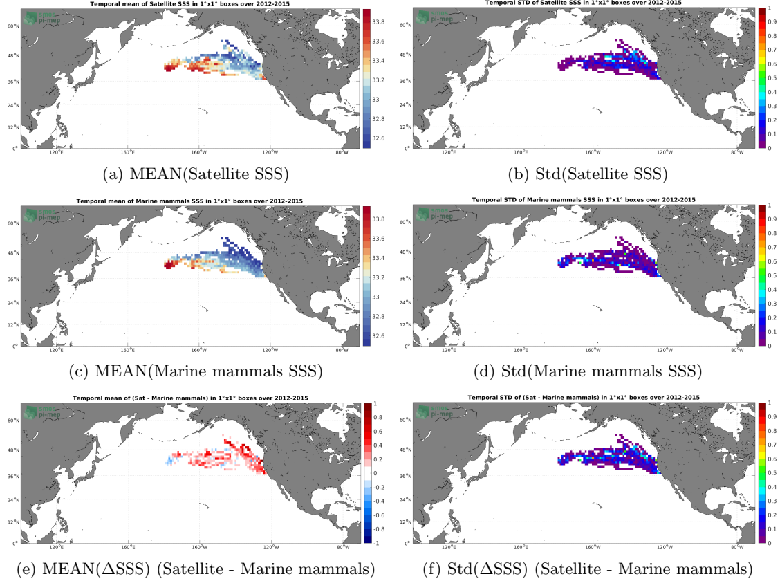
Figure 6: Temporal mean (left) and Std (right) of SSS from Aquarius SSS L3 CAP v5 - Monthly (JPL) (top), Marine mammals (middle), and of \Delta SSS (Satellite - Marine mammals). Only match-up pairs are used to generate these maps.
