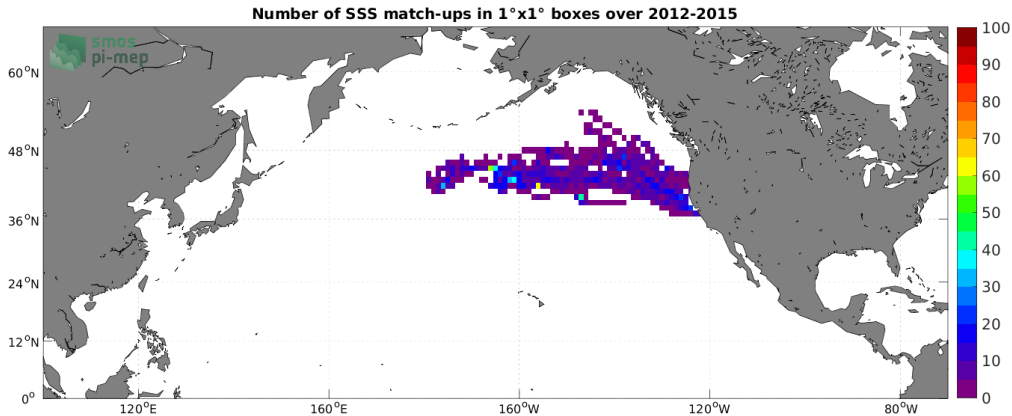
Figure 4: Number of SSS match-ups between Marine mammals SSS and the Aquarius SSS L3 CAP v5 - Monthly (JPL) SSS product for the North Pacific Ocean Pi-MEP region over 1^\circ \times 1^\circ boxes and for the full satellite product period.
