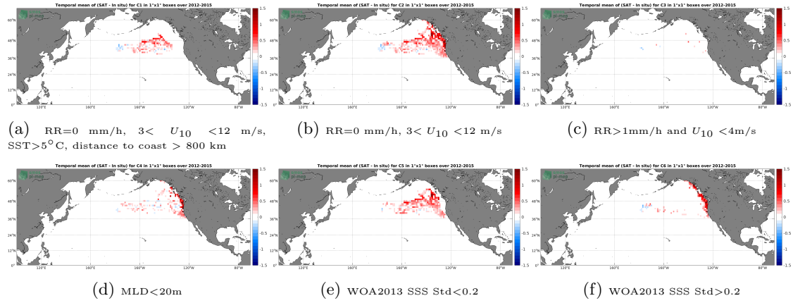
Figure 12: Temporal mean gridded over spatial boxes of size 1^\circ \times 1^\circ of \Delta SSS (Aquarius SSS L3 CAP v5 - Monthly (JPL) - Sea mammals) for 6 different subdatasets corresponding to: RR=0 mm/h, 3 < U_{10} < 12 m/s, SST > 5^\circ C , distance to coast > 800 km (a), RR=0 mm/h, 3 < U_{10} < 12 m/s (b), RR > 1 mm/h and U_{10} < 4 m/s (c), MLD < 20 m (d), WOA2013 SSS Std < 0.2 (e), WOA2013 SSS Std > 0.2 (f).
