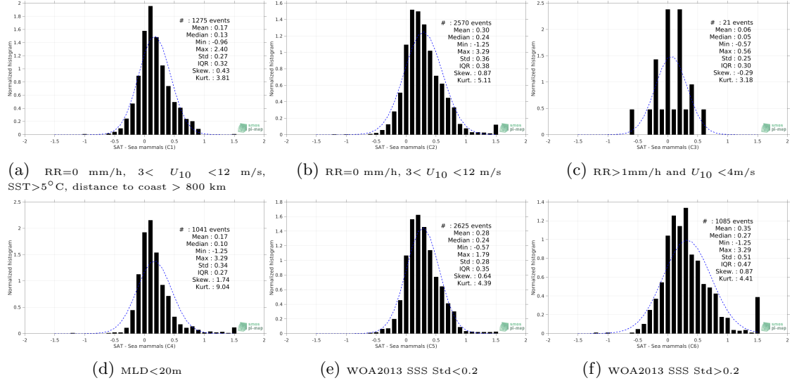
Figure 13: Normalized histogram of \Delta SSS (Aquarius SSS L3 CAP v5 - Monthly (JPL) - Sea mammals) for 6 different subdatasets corresponding to: RR=0 mm/h, 3 < U_{10} < 12 m/s, SST>5°C, distance to coast > 800 km (a), RR=0 mm/h, 3 < U_{10} < 12 m/s (b), RR>1mm/h and U_{10} < 4 m/s (c), MLD<20m (d), WOA2013 SSS Std<0.2 (e), WOA2013 SSS Std>0.2 (f).
