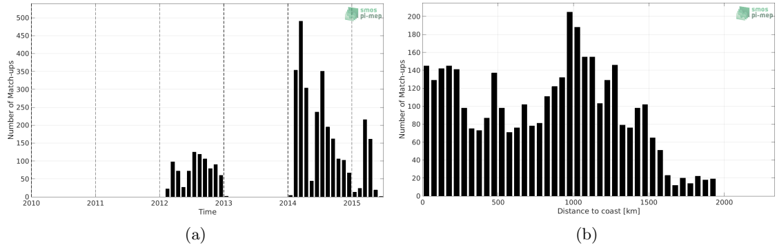
Figure 1: Number of match-ups between Sea mammals and Aquarius SSS L3 CAP v5 - Monthly (JPL) SSS as a function of time (a) and as function of the distance to coast (b) over the North Pacific Ocean Pi-MEP region and for the full satellite product period.
