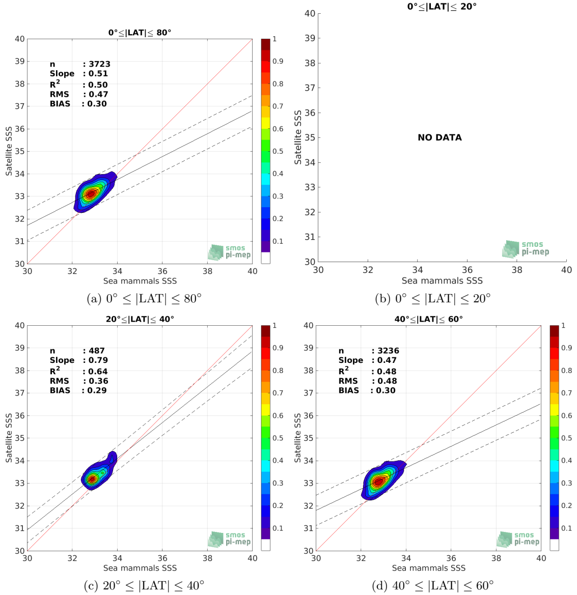
Figure 9: Contour maps of the concentration of Aquarius SSS L3 CAP v5 - Monthly (JPL) SSS (y-axis) versus Sea mammals SSS (x-axis) at match-up pairs for different latitude bands. For each plot, the red line shows x=y . The black thin and dashed lines indicate a linear fit through the data cloud and the \pm 95\% confidence levels, respectively. The number match-up pairs n , the slope and R^2 coefficient of the linear fit, the root mean square (RMS) and the mean bias between satellite and in situ data are indicated for each latitude band in each plots.
