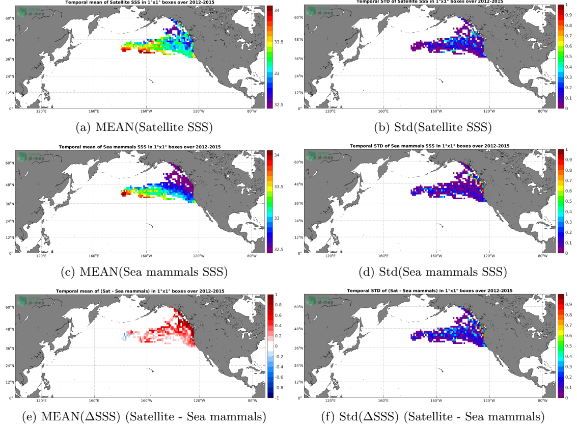
Figure 6: Temporal mean (left) and Std (right) of SSS from Aquarius SSS L3 CAP v5 - Monthly (JPL) (top), Sea mammals (middle), and of \Delta SSS (Satellite - Sea mammals). Only match-up pairs are used to generate these maps.
