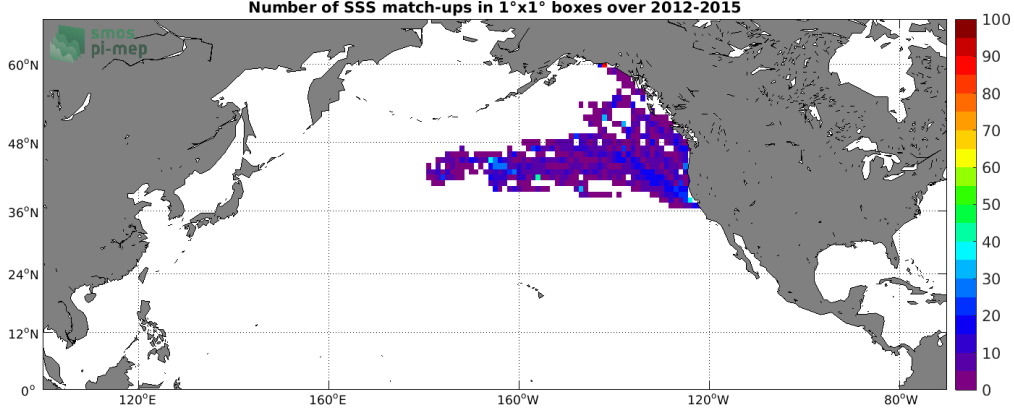
Figure 4: Number of SSS match-ups between Sea mammals SSS and the Aquarius SSS L3 CAP v5 - Monthly (JPL) SSS product for the North Pacific Ocean Pi-MEP region over 1^\circ \times 1^\circ boxes and for the full satellite product period.
