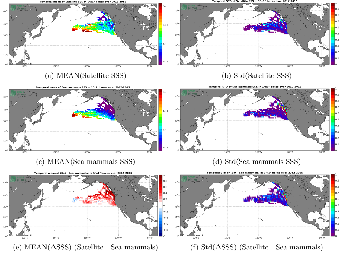
Figure 6: Temporal mean (left) and Std (right) of SSS from Aquarius-L3-JPL-V5-MONTHLY (top), Sea mammals (middle), and of \Delta SSS (Satellite - Sea mammals). Only match-up pairs are used to generate these maps.
