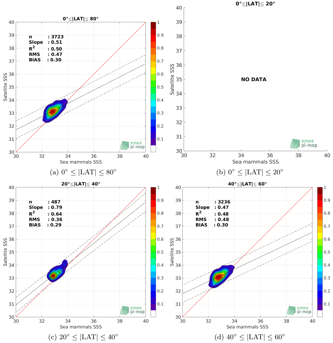
Figure 9: Contour maps of the concentration of Aquarius-L3-JPL-V5-MONTHLY SSS (y-axis) versus Sea mammals SSS (x-axis) at match-up pairs for different latitude bands. For each plot, the red line shows x=y . The black thin and dashed lines indicate a linear fit through the data cloud and the \pm 95\% confidence levels, respectively. The number match-up pairs n , the slope and R^2 coefficient of the linear fit, the root mean square (RMS) and the mean bias between satellite and in situ data are indicated for each latitude band in each plots.
