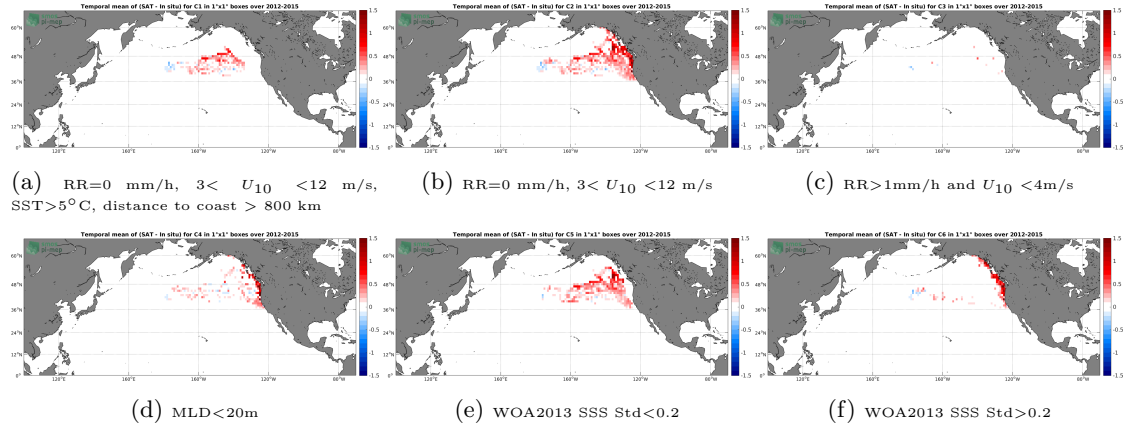
Figure 12: Temporal mean gridded over spatial boxes of size 1^\circ \times 1^\circ of \Delta SSS (Aquarius-L3-JPL-V5-MONTHLY - Sea mammals) for 6 different subdatasets corresponding to: RR=0 mm/h, 3 < U_{10} < 12 m/s, SST >5^\circ\text{C} , distance to coast > 800 km (a), RR=0 mm/h, 3 < U_{10} < 12 m/s (b), RR>1 mm/h and U_{10} < 4 m/s (c), MLD <20 m (d), WOA2013 SSS Std <0.2 (e), WOA2013 SSS Std >0.2 (f).
