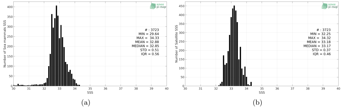
Figure 2: Histograms of SSS from Sea mammals (a) and Aquarius-L3-JPL-V5-MONTHLY (b) considering all match-up pairs per bins of 0.1 over the North Pacific Ocean Pi-MEP region and for the full satellite product period.
