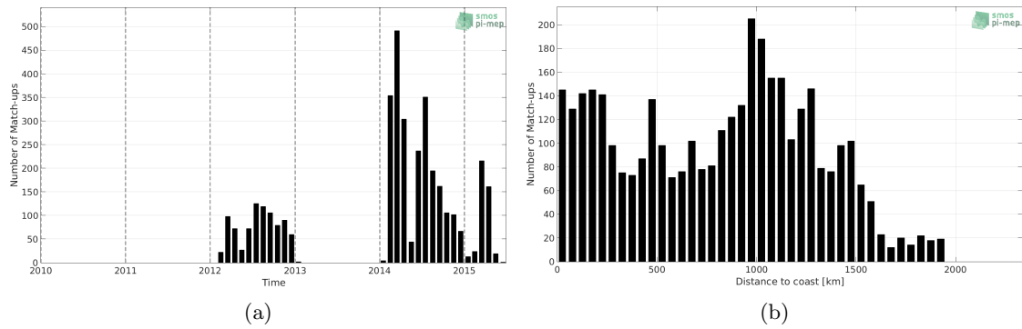
Figure 1: Number of match-ups between Sea mammals and Aquarius-L3-JPL-V5-MONTHLY SSS as a function of time (a) and as function of the distance to coast (b) over the North Pacific Ocean Pi-MEP region and for the full satellite product period.
