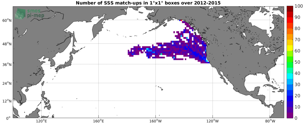
Figure 4: Number of SSS match-ups between Sea mammals SSS and the Aquarius-L3-JPL-V5-MONTHLY SSS product for the North Pacific Ocean Pi-MEP region over 1^\circ \times 1^\circ boxes and for the full satellite product period.
