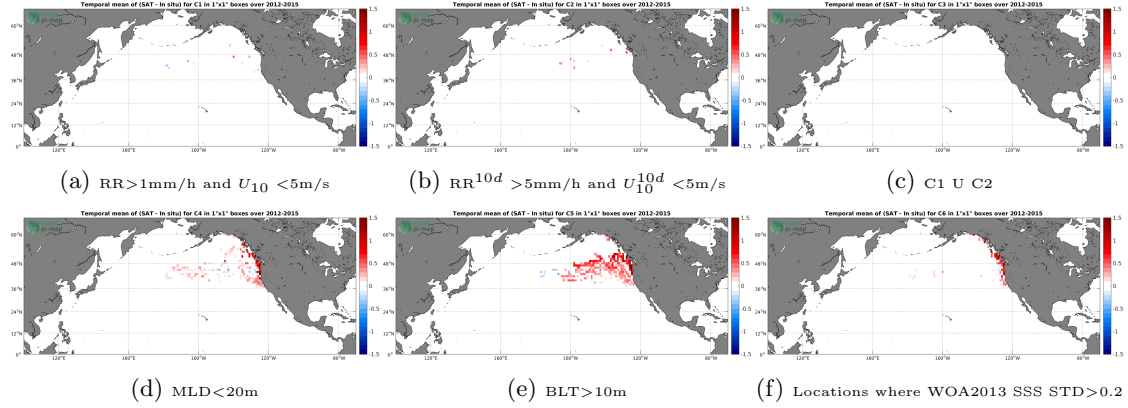
Figure 12: Temporal mean gridded over spatial boxes of size 1^\circ \times 1^\circ of \Delta SSS (Aquarius-L3-JPL-V5-MONTHLY - Sea mammals) for 6 different subdatasets corresponding to: RR > 1\text{mm/h} and U_{10} < 5\text{m/s} (a), RR^{10d} > 5\text{mm/h} and U_{10}^{10d} < 5\text{m/s} (b), C1 U C2 (c), MLD < 20\text{m} (d), BLT > 10\text{m} (e), Locations where WOA2013 SSS STD > 0.2 (f).
