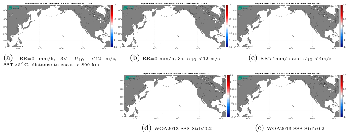
Figure 13: Temporal mean gridded over spatial boxes of size 1^\circ \times 1^\circ of \Delta SSS (Aquarius SSS L3 CAP v5 - Monthly (JPL) - Surface drifters) for 5 different subdatasets corresponding to:RR=0 mm/h, 3 < U_{10} < 12 m/s, SST >5^\circ C, distance to coast > 800 km (a), RR=0 mm/h, 3 < U_{10} < 12 m/s (b), RR >1 mm/h and U_{10} < 4 m/s (c), WOA2013 SSS Std <0.2 (d), WOA2013 SSS Std >0.2 (e).
