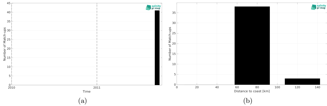
Figure 2: Number of match-ups between Surface drifters and Aquarius SSS L3 CAP v5 - Monthly (JPL) SSS as a function of time (a) and as function of the distance to coast (b) over the North Pacific Ocean Pi-MEP region and for the full satellite product period.
