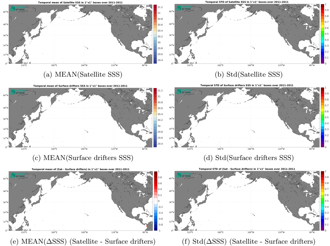
Figure 6: Temporal mean (left) and Std (right) of SSS from Aquarius SSS L3 CAP v5 - Monthly (JPL) (top), Surface drifters (middle), and of \Delta SSS (Satellite - Surface drifters). Only match-up pairs are used to generate these maps.
