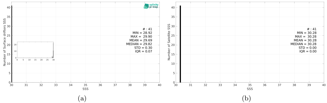
Figure 3: Histograms of SSS from Surface drifters (a) and Aquarius SSS L3 CAP v5 - Monthly (JPL) (b) considering all match-up pairs per bins of 0.1 over the North Pacific Ocean Pi-MEP region and for the full satellite product period.
