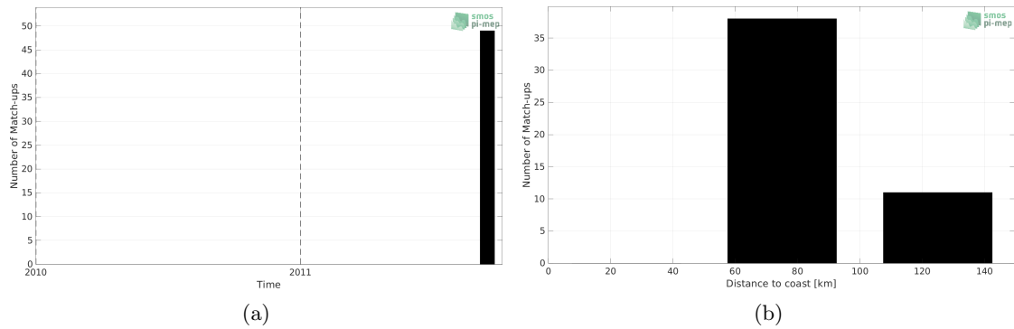
Figure 1: Number of match-ups between Surface drifters and Aquarius SSS L3 CAP v5 - Monthly (JPL) SSS as a function of time (a) and as function of the distance to coast (b) over the North Pacific Ocean Pi-MEP region and for the full satellite product period.
