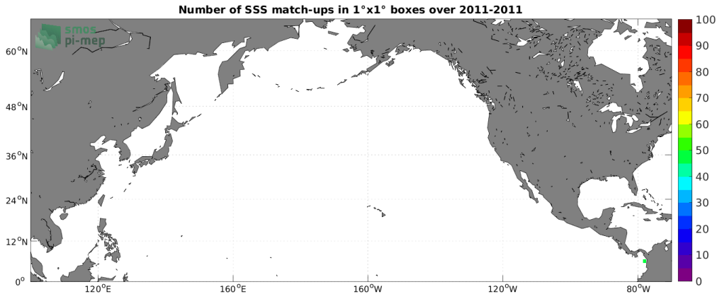
Figure 3: Number of SSS match-ups between Surface drifters SSS and the Aquarius SSS L3 CAP v5 - Monthly (JPL) SSS product for the North Pacific Ocean Pi-MEP region over 1^\circ \times 1^\circ boxes and for the full satellite product period.
