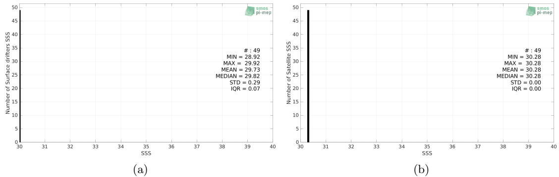
Figure 2: Histograms of SSS from Surface drifters (a) and Aquarius SSS L3 CAP v5 - Monthly (JPL) (b) considering all match-up pairs per bins of 0.1 over the North Pacific Ocean Pi-MEP region and for the full satellite product period.
