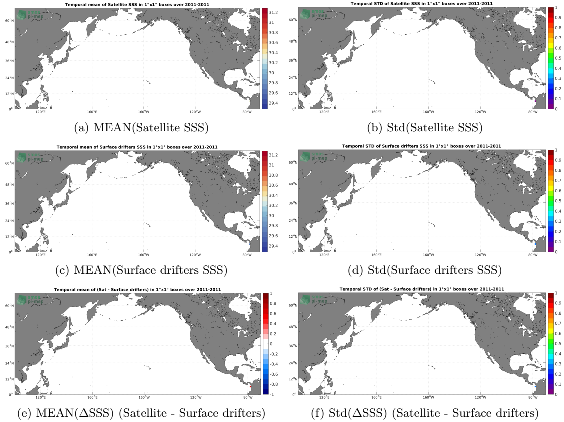
Figure 5: Temporal mean (left) and Std (right) of SSS from Aquarius SSS L3 CAP v5 - Monthly (JPL) (top), Surface drifters (middle), and of \Delta SSS (Satellite - Surface drifters). Only match-up pairs are used to generate these maps.
