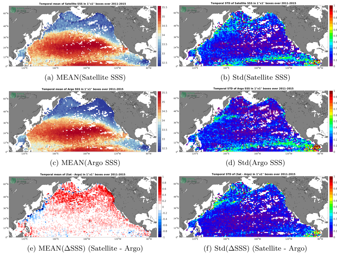
Figure 6: Temporal mean (left) and Std (right) of SSS from Aquarius SSS L3 CAP v5 - Monthly (JPL) (top), Argo (middle), and of \Delta SSS (Satellite - Argo). Only match-up pairs are used to generate these maps.
