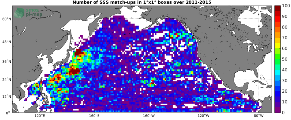
Figure 4: Number of SSS match-ups between Argo SSS and the Aquarius-L3-JPL-V5-MONTHLY SSS product for the North Pacific Ocean Pi-MEP region over 1^\circ \times 1^\circ boxes and for the full satellite product period.
