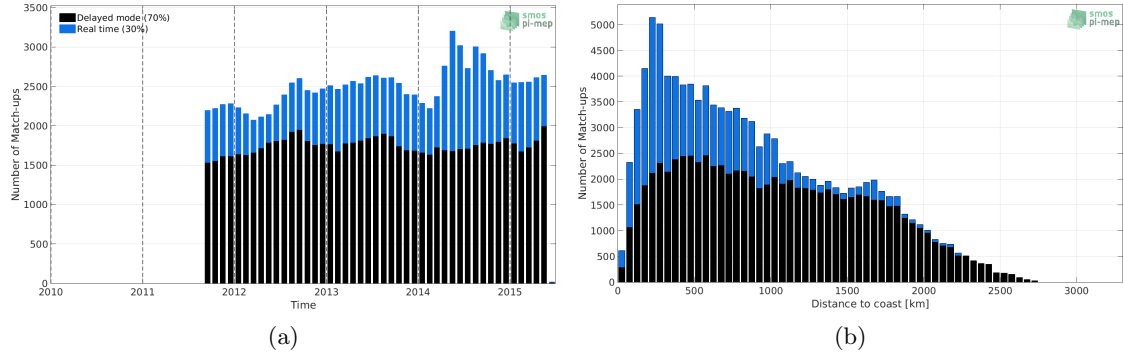
Figure 1: Number of match-ups between Argo and Aquarius-L3-JPL-V5-MONTHLY SSS as a function of time (a) and as function of the distance to coast (b) over the North Pacific Ocean Pi-MEP region and for the full satellite product period.
