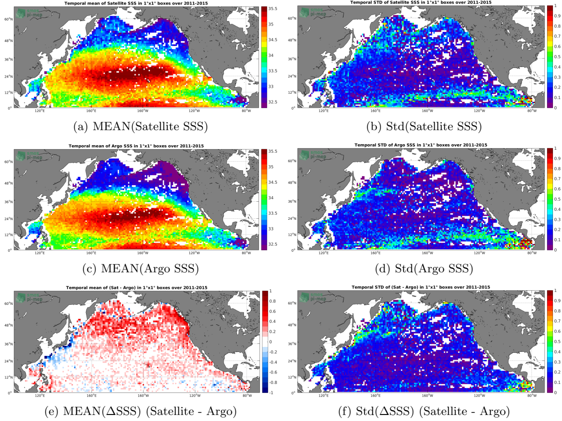
Figure 6: Temporal mean (left) and Std (right) of SSS from Aquarius-L3-JPL-V5-MONTHLY (top), Argo (middle), and of \Delta SSS (Satellite - Argo). Only match-up pairs are used to generate these maps.
