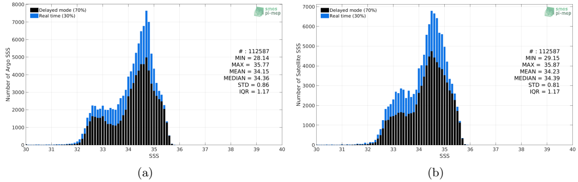
Figure 2: Histograms of SSS from Argo (a) and Aquarius-L3-JPL-V5-MONTHLY (b) considering all match-up pairs per bins of 0.1 over the North Pacific Ocean Pi-MEP region and for the full satellite product period.
