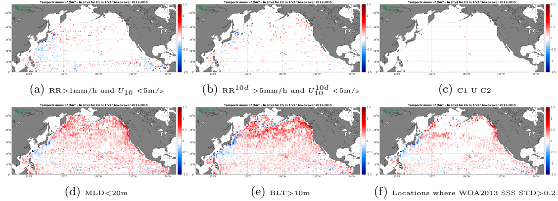
Figure 12: Temporal mean gridded over spatial boxes of size 1^\circ \times 1^\circ of \Delta\text{SSS} (Aquarius-L3-JPL-V5-MONTHLY - Argo) for 6 different subdatasets corresponding to: \text{RR} > 1\text{mm/h} and U_{10} < 5\text{m/s} (a), \text{RR}^{10d} > 5\text{mm/h} and U_{10}^{10d} < 5\text{m/s} (b), C1 U C2 (c), \text{MLD} < 20\text{m} (d), \text{BLT} > 10\text{m} (e), Locations where WOA2013 SSS STD > 0.2 (f).
