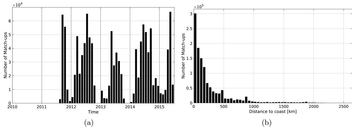
Figure 1: Number of match-ups between TSG-SAMOS and Aquarius-L3-JPL-V4-7DAY-RUNNING SSS as a function of time (a) and as function of the distance to coast (b) over the North Pacific Ocean Pi-MEP region and for the full satellite product period.
