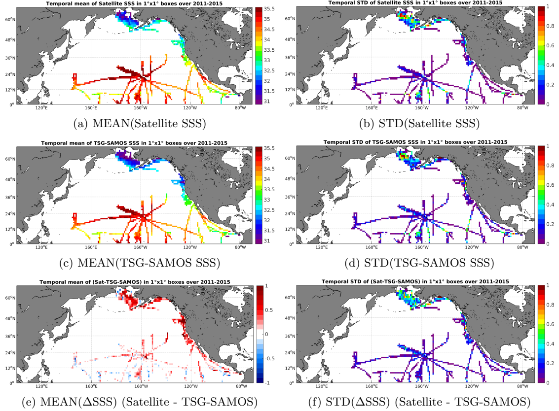
Figure 6: Temporal mean (left) and STD (right) of SSS from Aquarius-L3-JPL-V4-7DAY-RUNNING (top), TSG-SAMOS (middle), and of \Delta SSS (Satellite - TSG-SAMOS). Only match-up pairs are used to generate these maps.
