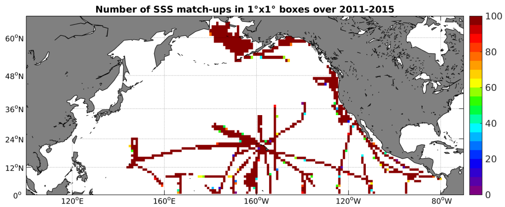
Figure 4: Number of SSS match-ups between TSG-SAMOS SSS and the Aquarius-L3-JPL-V4-7DAY-RUNNING SSS product for the North Pacific Ocean Pi-MEP region over 1^\circ \times 1^\circ boxes and for the full satellite product period.
