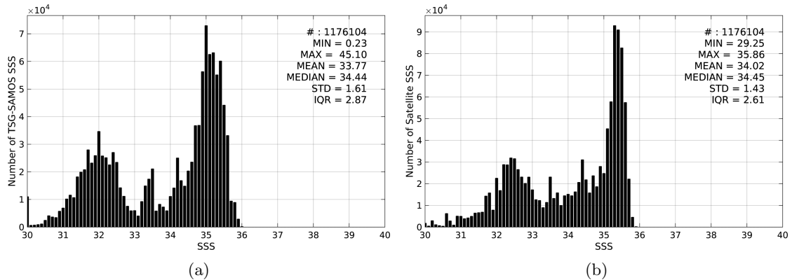
Figure 2: Histograms of SSS from TSG-SAMOS (a) and Aquarius-L3-JPL-V4-7DAY-RUNNING (b) considering all match-up pairs per bins of 0.1 over the North Pacific Ocean Pi-MEP region and for the full satellite product period.
