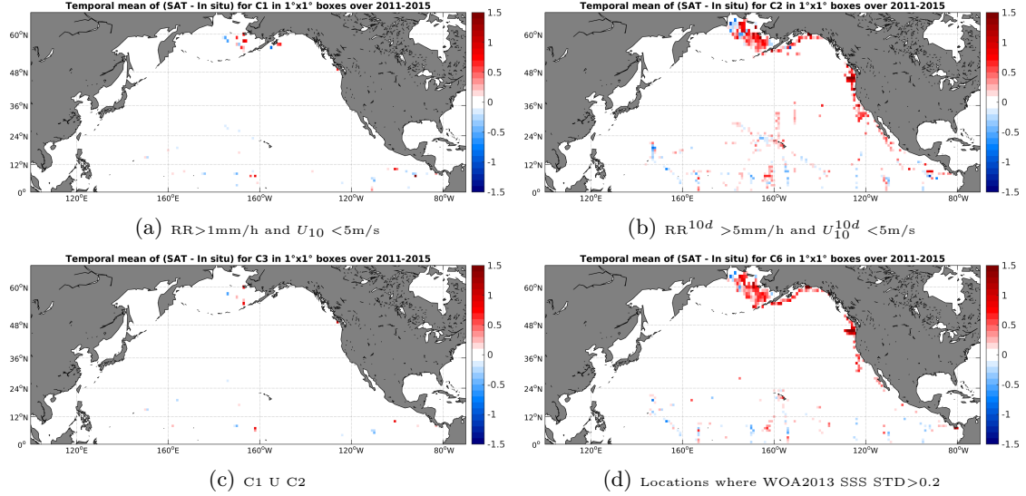
Figure 12: Temporal mean gridded over spatial boxes of size 1^\circ \times 1^\circ of \Delta SSS (Aquarius-L3-JPL-V4-7DAY-RUNNING - TSG-SAMOS) for 4 different subdatasets corresponding to: RR > 1mm/h and U_{10} < 5 m/s (a), RR^{10d} > 5 mm/h and U_{10}^{10d} < 5 m/s (b), C1 U C2 (c), Locations where WOA2013 SSS STD > 0.2 (d).
