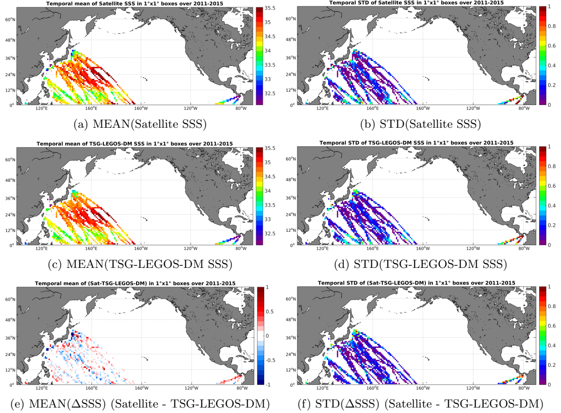
Figure 6: Temporal mean (left) and STD (right) of SSS from Aquarius-L3-JPL-V4-7DAY-RUNNING (top), TSG-LEGOS-DM (middle), and of \Delta SSS (Satellite - TSG-LEGOS-DM). Only match-up pairs are used to generate these maps.
