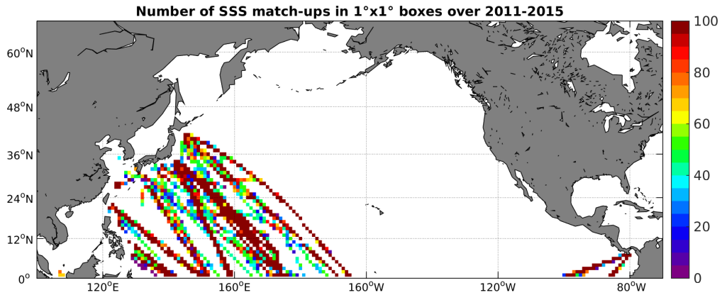
Figure 4: Number of SSS match-ups between TSG-LEGOS-DM SSS and the Aquarius-L3-JPL-V4-7DAY-RUNNING SSS product for the North Pacific Ocean Pi-MEP region over 1^\circ \times 1^\circ boxes and for the full satellite product period.
