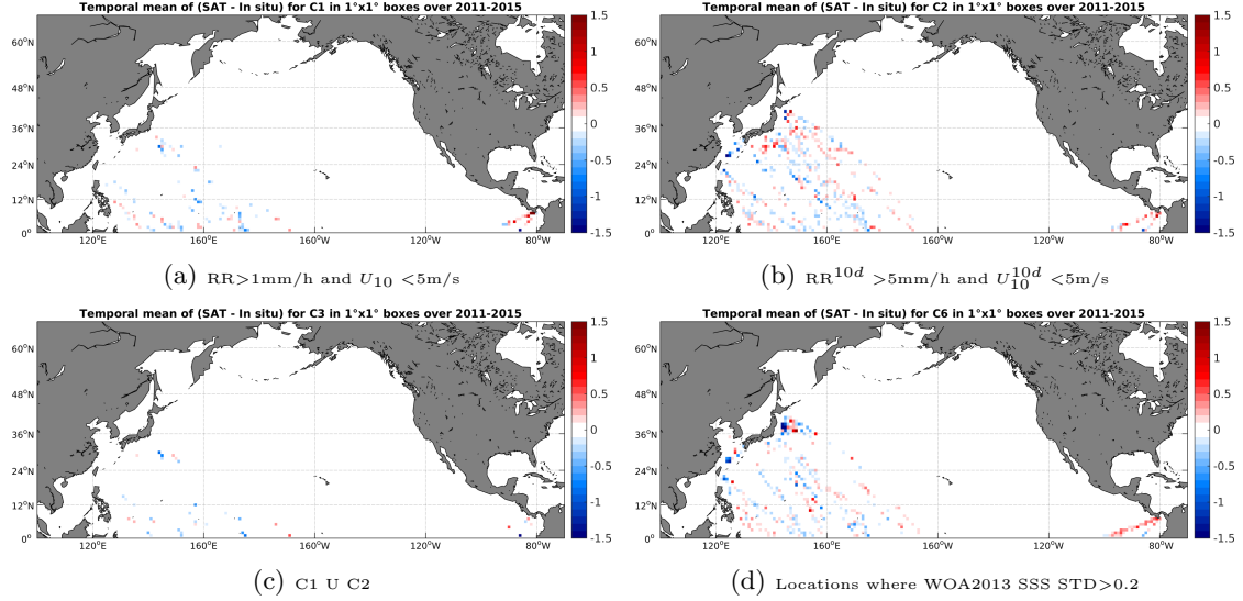
Figure 12: Temporal mean gridded over spatial boxes of size 1^\circ \times 1^\circ of \Delta SSS (Aquarius-L3-JPL-V4-7DAY-RUNNING - TSG-LEGOS-DM) for 4 different subdatasets corresponding to: RR > 1 mm/h and U_{10} < 5 m/s (a), RR^{10d} > 5 mm/h and U_{10}^{10d} < 5 m/s (b), C1 U C2 (c), Locations where WOA2013 SSS STD > 0.2 (d).
