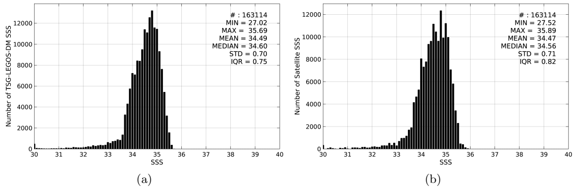
Figure 2: Histograms of SSS from TSG-LEGOS-DM (a) and Aquarius-L3-JPL-V4-7DAY-RUNNING (b) considering all match-up pairs per bins of 0.1 over the North Pacific Ocean Pi-MEP region and for the full satellite product period.
