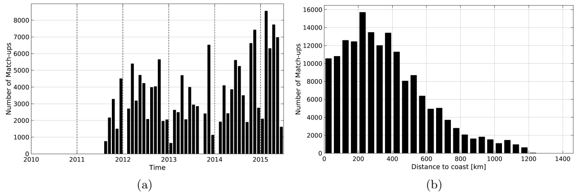
Figure 1: Number of match-ups between TSG-LEGOS-DM and Aquarius-L3-JPL-V4-7DAY-RUNNING SSS as a function of time (a) and as function of the distance to coast (b) over the North Pacific Ocean Pi-MEP region and for the full satellite product period.
