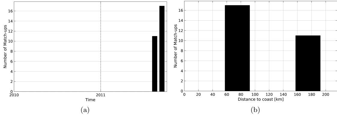
Figure 1: Number of match-ups between Surface drifters and Aquarius-L3-JPL-V4-7DAY-RUNNING SSS as a function of time (a) and as function of the distance to coast (b) over the North Pacific Ocean Pi-MEP region and for the full satellite product period.
