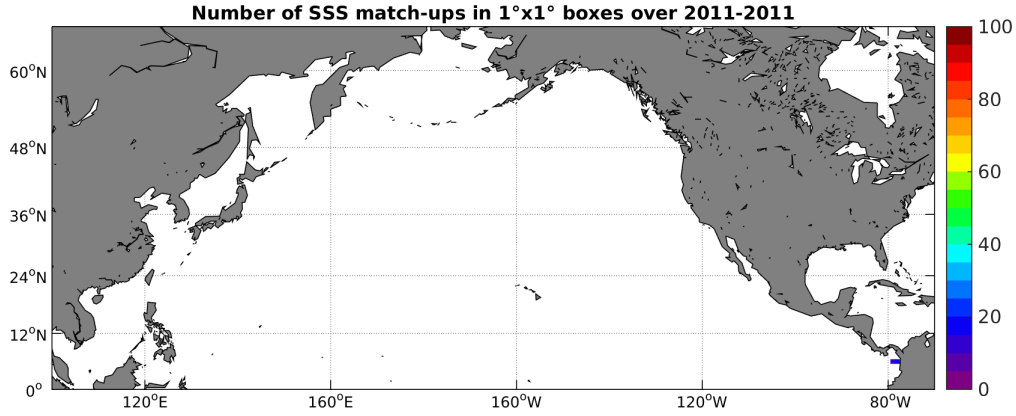
Figure 3: Number of SSS match-ups between Surface drifters SSS and the Aquarius-L3-JPL-V4-7DAY-RUNNING SSS product for the North Pacific Ocean Pi-MEP region over 1^\circ \times 1^\circ boxes and for the full satellite product period.
