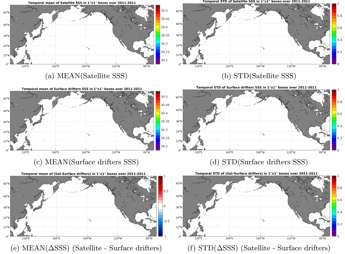
Figure 5: Temporal mean (left) and STD (right) of SSS from Aquarius-L3-JPL-V4-7DAY-RUNNING (top), Surface drifters (middle), and of \Delta SSS (Satellite - Surface drifters). Only match-up pairs are used to generate these maps.
