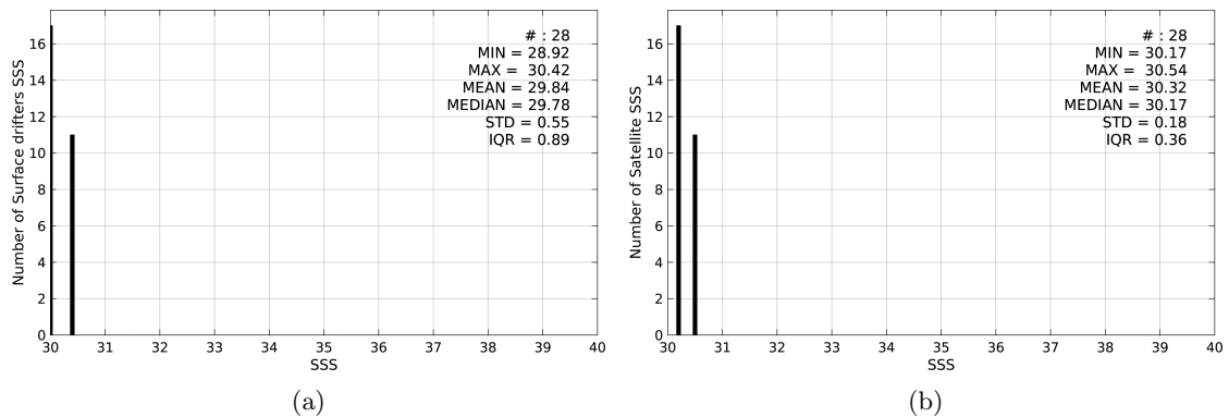
Figure 2: Histograms of SSS from Surface drifters (a) and Aquarius-L3-JPL-V4-7DAY-RUNNING (b) considering all match-up pairs per bins of 0.1 over the North Pacific Ocean Pi-MEP region and for the full satellite product period.
