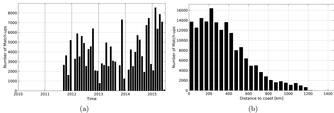
Figure 1: Number of match-ups between TSG-LEGOS-DM and Aquarius-L3-JPL-V4-MONTHLY SSS as a function of time (a) and as function of the distance to coast (b) over the North Pacific Ocean Pi-MEP region and for the full satellite product period.
