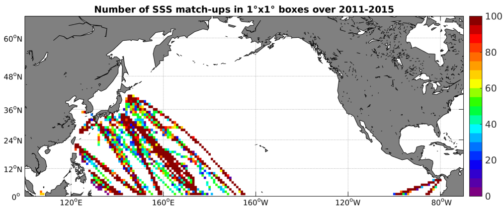
Figure 4: Number of SSS match-ups between TSG-LEGOS-DM SSS and the Aquarius-L3-JPL-V4-MONTHLY SSS product for the North Pacific Ocean Pi-MEP region over 1^\circ \times 1^\circ boxes and for the full satellite product period.
