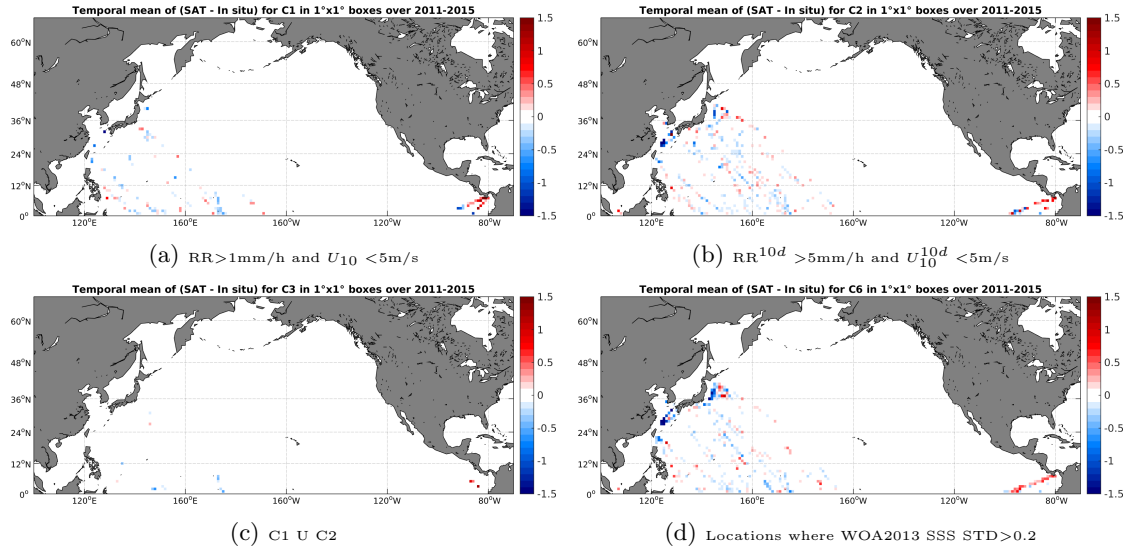
Figure 12: Temporal mean gridded over spatial boxes of size 1^\circ \times 1^\circ of \Delta SSS (Aquarius-L3-JPL-V4-MONTHLY - TSG-LEGOS-DM) for 4 different subdatasets corresponding to: RR > 1\text{mm/h} and U_{10} < 5\text{m/s} (a), RR^{10d} > 5\text{mm/h} and U_{10}^{10d} < 5\text{m/s} (b), C1 U C2 (c), Locations where WOA2013 SSS STD > 0.2 (d).
