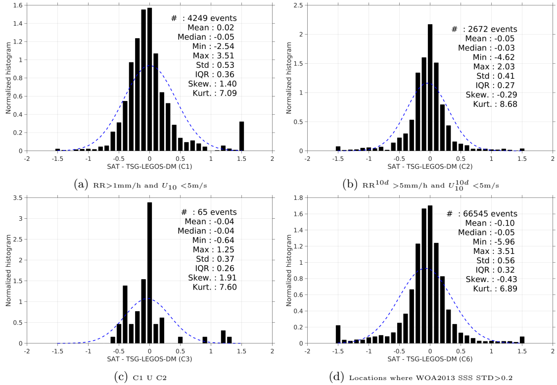
Figure 13: Normalized histogram of \Delta SSS (Aquarius-L3-JPL-V4-MONTHLY - TSG-LEGOS-DM) for 6 different subdatasets corresponding to: RR > 1\text{mm/h} and U_{10} < 5\text{m/s} (a), RR^{10d} > 5\text{mm/h} and U_{10}^{10d} < 5\text{m/s} (b), C1 U C2 (c), Locations where WOA2013 SSS STD > 0.2 (d).
