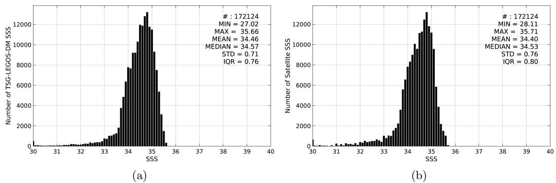
Figure 2: Histograms of SSS from TSG-LEGOS-DM (a) and Aquarius-L3-JPL-V4-MONTHLY (b) considering all match-up pairs per bins of 0.1 over the North Pacific Ocean Pi-MEP region and for the full satellite product period.
