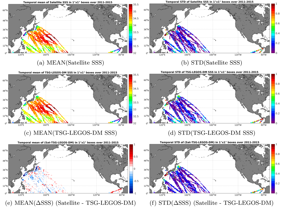
Figure 6: Temporal mean (left) and STD (right) of SSS from Aquarius-L3-JPL-V4-MONTHLY (top), TSG-LEGOS-DM (middle), and of \Delta SSS (Satellite - TSG-LEGOS-DM). Only match-up pairs are used to generate these maps.
