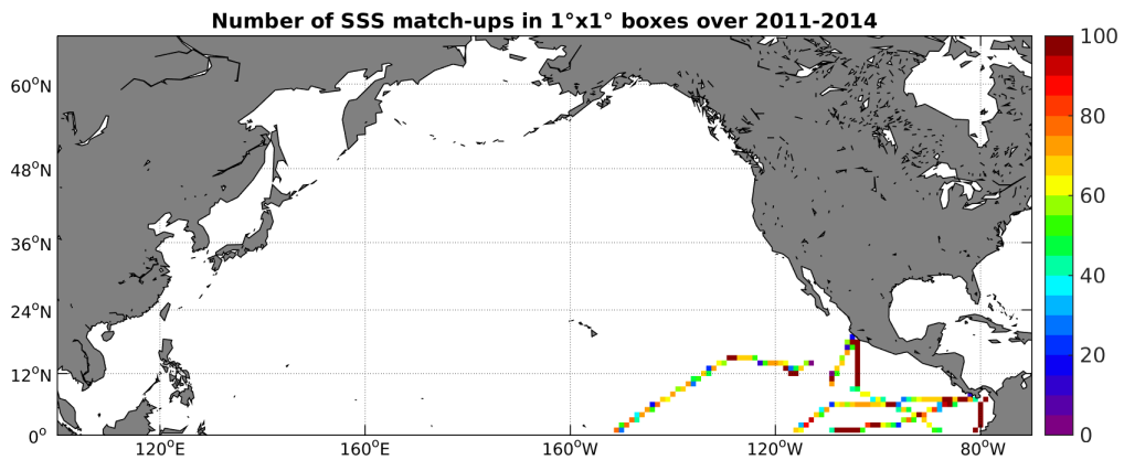
Figure 4: Number of SSS match-ups between TSG-GOSUD-Research-vessel SSS and the Aquarius-L3-JPL-V4-MONTHLY SSS product for the North Pacific Ocean Pi-MEP region over 1^\circ \times 1^\circ boxes and for the full satellite product period.
