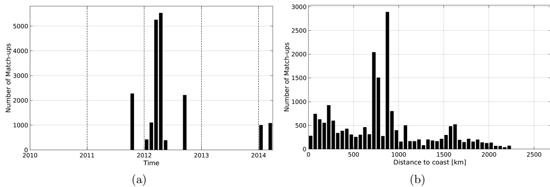
Figure 1: Number of match-ups between TSG-GOSUD-Research-vessel and Aquarius-L3-JPL-V4-MONTHLY SSS as a function of time (a) and as function of the distance to coast (b) over the North Pacific Ocean Pi-MEP region and for the full satellite product period.
