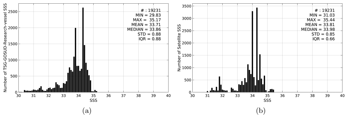
Figure 2: Histograms of SSS from TSG-GOSUD-Research-vessel (a) and Aquarius-L3-JPL-V4-MONTHLY (b) considering all match-up pairs per bins of 0.1 over the North Pacific Ocean Pi-MEP region and for the full satellite product period.
