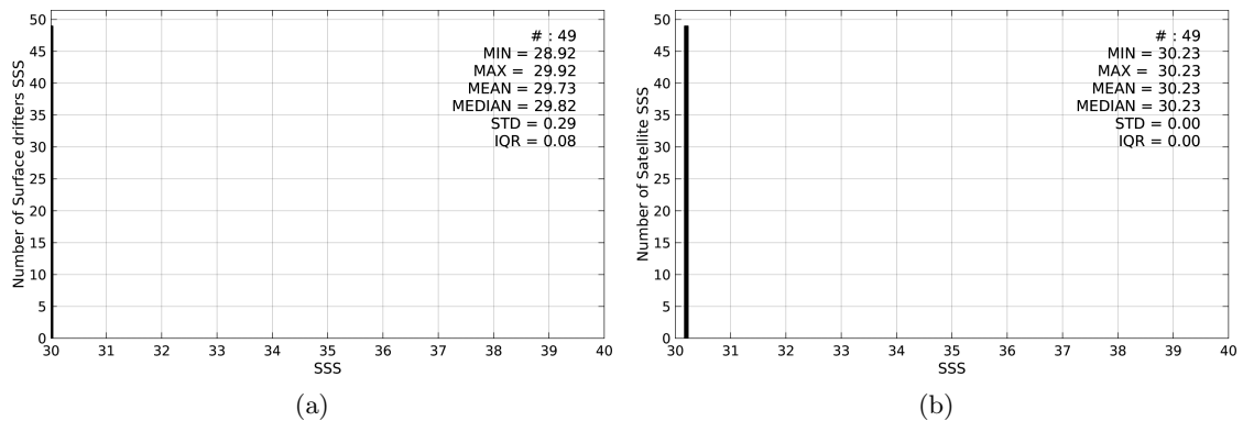
Figure 2: Histograms of SSS from Surface drifters (a) and Aquarius-L3-JPL-V4-MONTHLY (b) considering all match-up pairs per bins of 0.1 over the North Pacific Ocean Pi-MEP region and for the full satellite product period.
