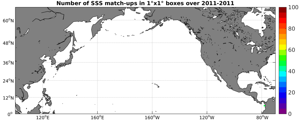
Figure 3: Number of SSS match-ups between Surface drifters SSS and the Aquarius-L3-JPL-V4-MONTHLY SSS product for the North Pacific Ocean Pi-MEP region over 1^\circ \times 1^\circ boxes and for the full satellite product period.
