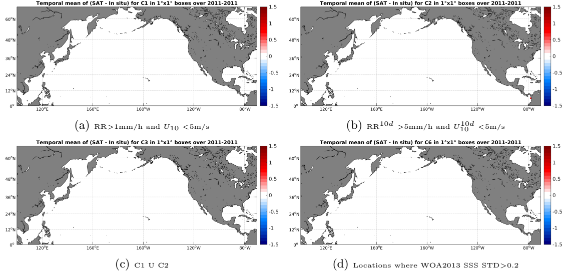
Figure 11: Temporal mean gridded over spatial boxes of size 1^\circ \times 1^\circ of \Delta SSS (Aquarius-L3-JPL-V4-MONTHLY - Surface drifters) for 4 different subdatasets corresponding to: RR > 1mm/h and U_{10} < 5 m/s (a), RR^{10d} > 5 mm/h and U_{10}^{10d} < 5 m/s (b), C1 U C2 (c), Locations where WOA2013 SSS STD > 0.2 (d).
