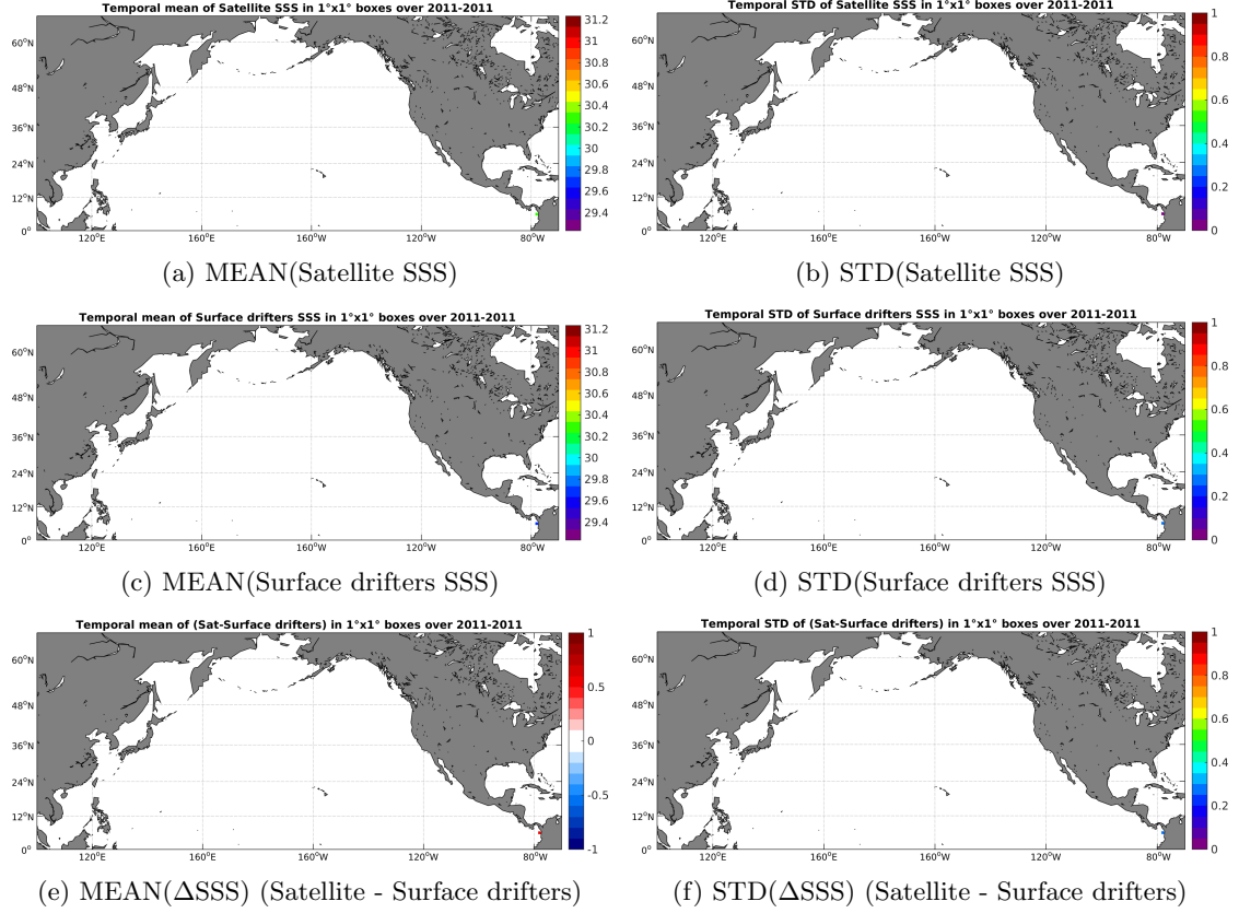
Figure 5: Temporal mean (left) and STD (right) of SSS from Aquarius-L3-JPL-V4-MONTHLY (top), Surface drifters (middle), and of \Delta SSS (Satellite - Surface drifters). Only match-up pairs are used to generate these maps.
