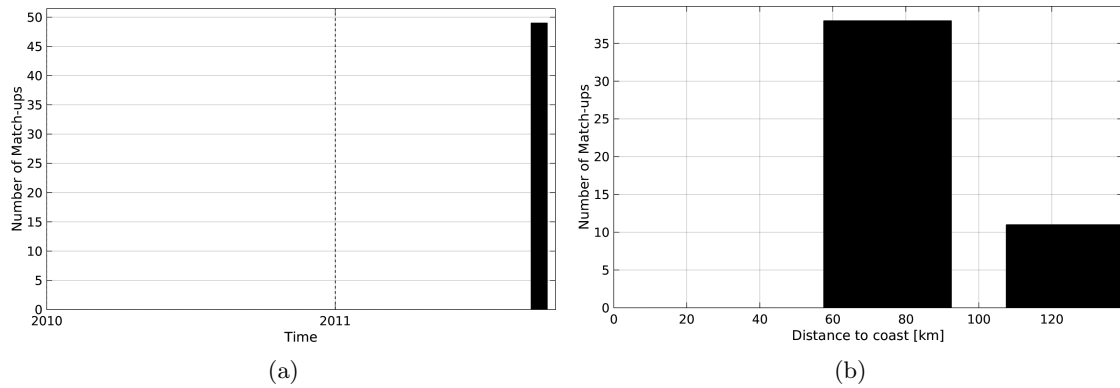
Figure 1: Number of match-ups between Surface drifters and Aquarius-L3-JPL-V4-MONTHLY SSS as a function of time (a) and as function of the distance to coast (b) over the North Pacific Ocean Pi-MEP region and for the full satellite product period.
