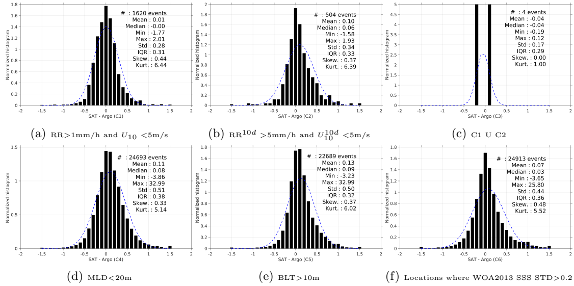
Figure 13: Normalized histogram of \Delta SSS (Aquarius-L3-JPL-V4-MONTHLY - Argo) for 6 different subdatasets corresponding to: RR>1mm/h and U_{10} < 5 m/s (a), RR^{10d} > 5 mm/h and U_{10}^{10d} < 5 m/s (b), C1 U C2 (c),MLD<20m (d),BLT>10m (e),Locations where WOA2013 SSS STD>0.2 (f).
