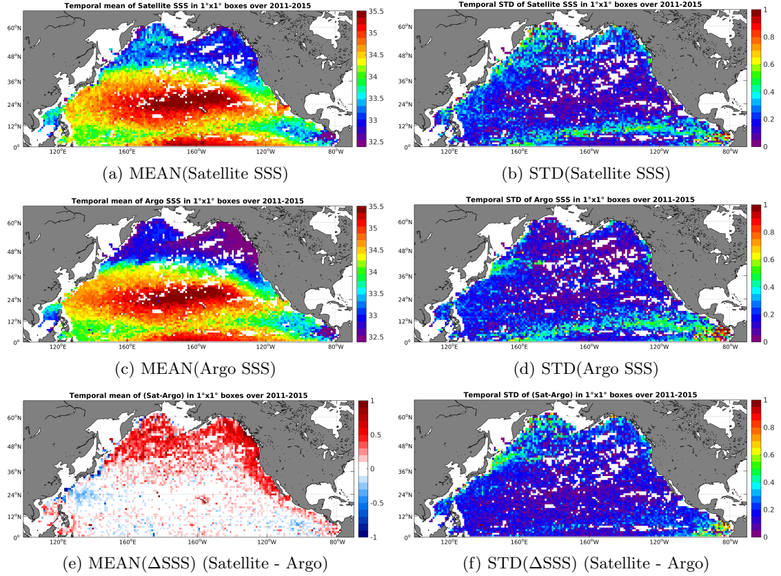
Figure 6: Temporal mean (left) and STD (right) of SSS from Aquarius-L3-JPL-V4-MONTHLY (top), Argo (middle), and of \Delta SSS (Satellite - Argo). Only match-up pairs are used to generate these maps.
