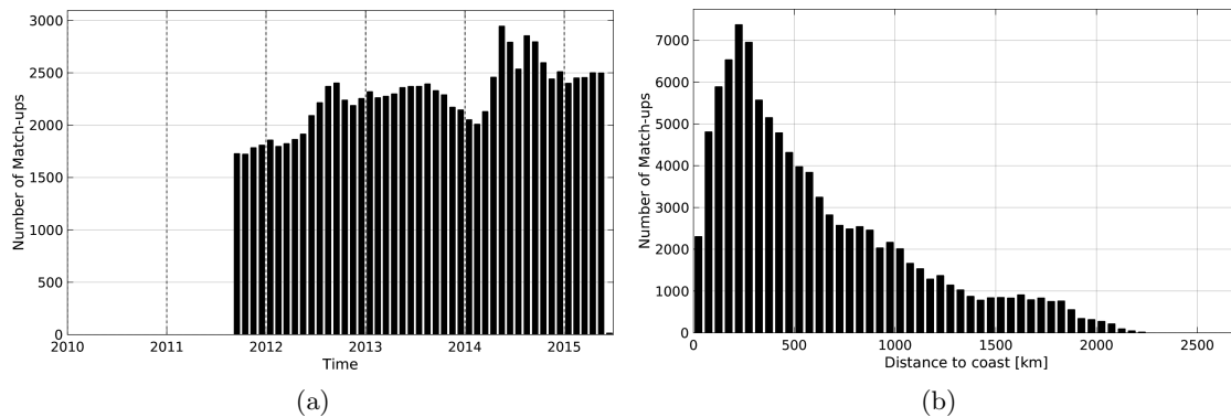
Figure 1: Number of match-ups between Argo and Aquarius-L3-JPL-V4-MONTHLY SSS as a function of time (a) and as function of the distance to coast (b) over the North Pacific Ocean Pi-MEP region and for the full satellite product period.
