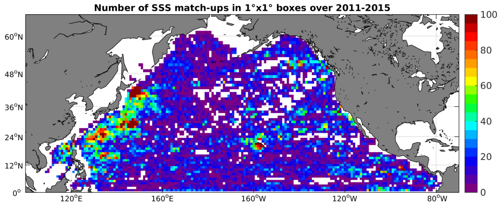
Figure 4: Number of SSS match-ups between Argo SSS and the Aquarius-L3-JPL-V4-MONTHLY SSS product for the North Pacific Ocean Pi-MEP region over 1^\circ \times 1^\circ boxes and for the full satellite product period.
