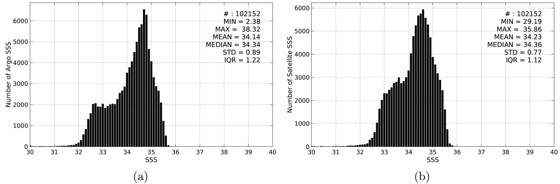
Figure 2: Histograms of SSS from Argo (a) and Aquarius-L3-JPL-V4-MONTHLY (b) considering all match-up pairs per bins of 0.1 over the North Pacific Ocean Pi-MEP region and for the full satellite product period.
