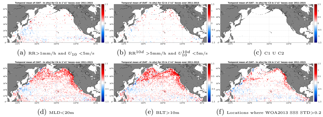
Figure 12: Temporal mean gridded over spatial boxes of size 1^\circ \times 1^\circ of \Delta SSS (Aquarius-L3-JPL-V4-MONTHLY - Argo) for 6 different subdatasets corresponding to: RR > 1\text{mm/h} and U_{10} < 5\text{m/s} (a), RR^{10d} > 5\text{mm/h} and U_{10}^{10d} < 5\text{m/s} (b), C1 U C2 (c), MLD < 20\text{m} (d), BLT > 10\text{m} (e), Locations where WOA2013 SSS STD > 0.2 (f).
