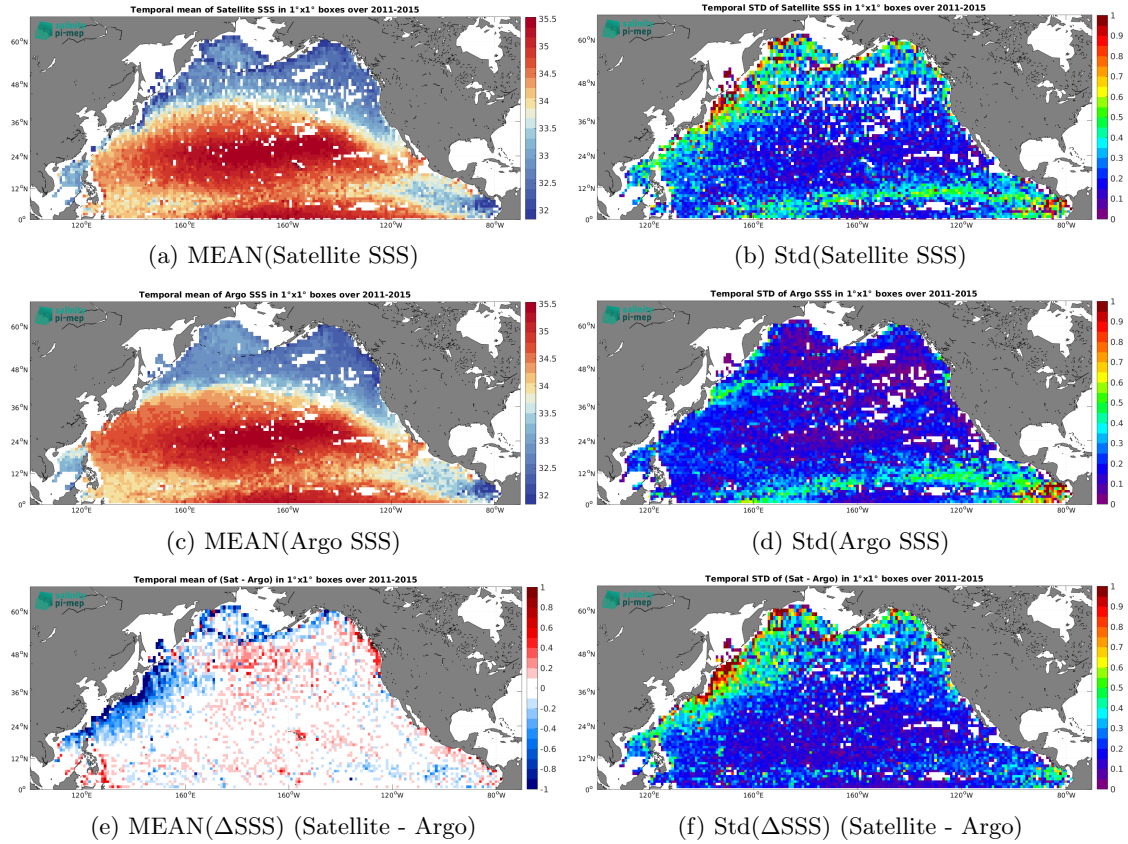
Figure 6: Temporal mean (left) and Std (right) of SSS from Aquarius SSS L2-AVERAGED OR v5 (NASA-GSFC) (top), Argo (middle), and of \Delta SSS (Satellite - Argo). Only match-up pairs are used to generate these maps.
