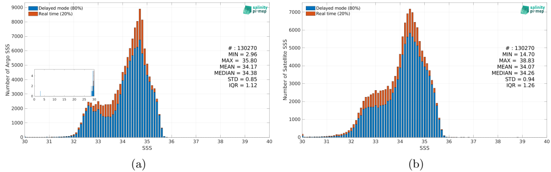
Figure 2: Histograms of SSS from Argo (a) and Aquarius SSS L2-AVERAGED OR v5 (NASA-GSFC) (b) considering all match-up pairs per bins of 0.1 over the North Pacific Ocean Pi-MEP region and for the full satellite product period.
