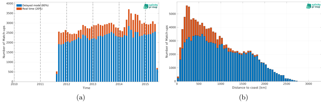
Figure 1: Number of match-ups between Argo and Aquarius SSS L2-AVERAGED OR v5 (NASA-GSFC) SSS as a function of time (a) and as function of the distance to coast (b) over the North Pacific Ocean Pi-MEP region and for the full satellite product period.
