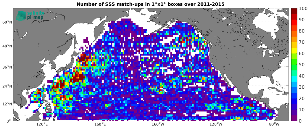
Figure 4: Number of SSS match-ups between Argo SSS and the Aquarius SSS L2-AVERAGED OR v5 (NASA-GSFC) SSS product for the North Pacific Ocean Pi-MEP region over 1^\circ \times 1^\circ boxes and for the full satellite product period.
