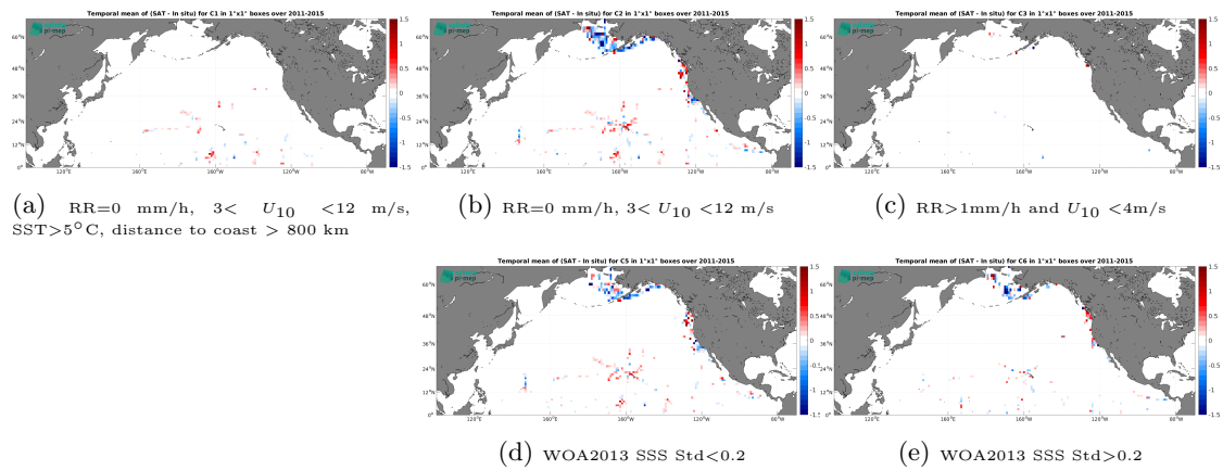
Figure 14: Temporal mean gridded over spatial boxes of size 1^\circ \times 1^\circ of \Delta SSS (Aquarius SSS L2 OR v5 (NASA-GSFC) - TSG (SAMOS)) for 5 different subdatasets corresponding to: RR=0 mm/h, 3 < U_{10} < 12 m/s, SST > 5°C, distance to coast > 800 km (a), RR=0 mm/h, 3 < U_{10} < 12 m/s (b), RR > 1 mm/h and U_{10} < 4 m/s (c), WOA2013 SSS Std < 0.2 (d), WOA2013 SSS Std > 0.2 (e).
