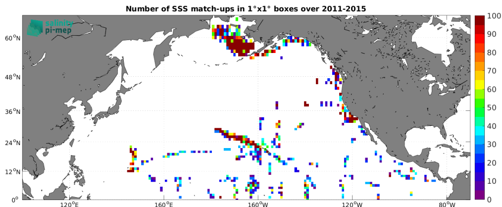
Figure 5: Number of SSS match-ups between TSG (SAMOS) SSS and the Aquarius SSS L2 OR v5 (NASA-GSFC) SSS product for the North Pacific Ocean Pi-MEP region over 1^\circ \times 1^\circ boxes and for the full satellite product period.
