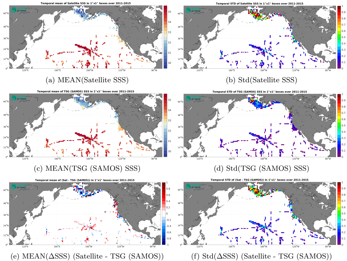
Figure 7: Temporal mean (left) and Std (right) of SSS from Aquarius SSS L2 OR v5 (NASA-GSFC) (top), TSG (SAMOS) (middle), and of \Delta SSS (Satellite - TSG (SAMOS)). Only match-up pairs are used to generate these maps.
