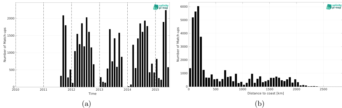
Figure 2: Number of match-ups between TSG (SAMOS) and Aquarius SSS L2 OR v5 (NASA-GSFC) SSS as a function of time (a) and as function of the distance to coast (b) over the North Pacific Ocean Pi-MEP region and for the full satellite product period.
