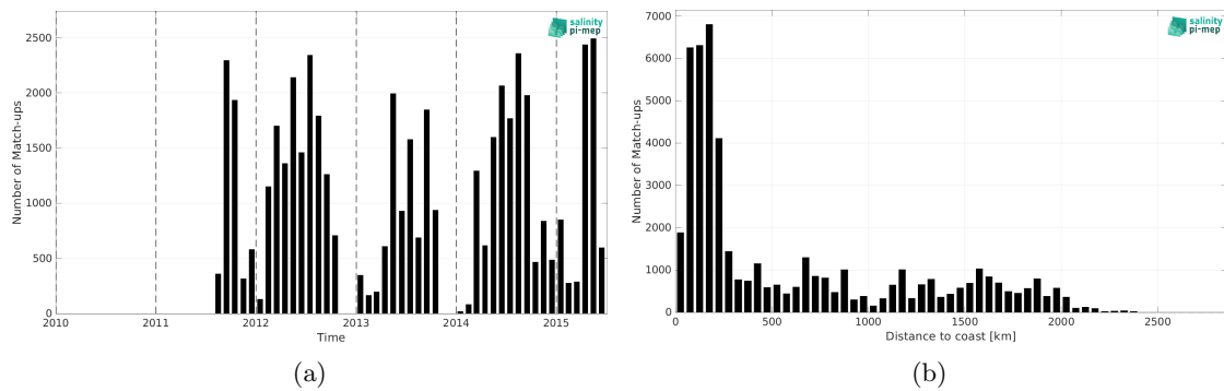
Figure 1: Number of match-ups between TSG (SAMOS) and Aquarius SSS L2 OR v5 (NASA-GSFC) SSS as a function of time (a) and as function of the distance to coast (b) over the North Pacific Ocean Pi-MEP region and for the full satellite product period.
