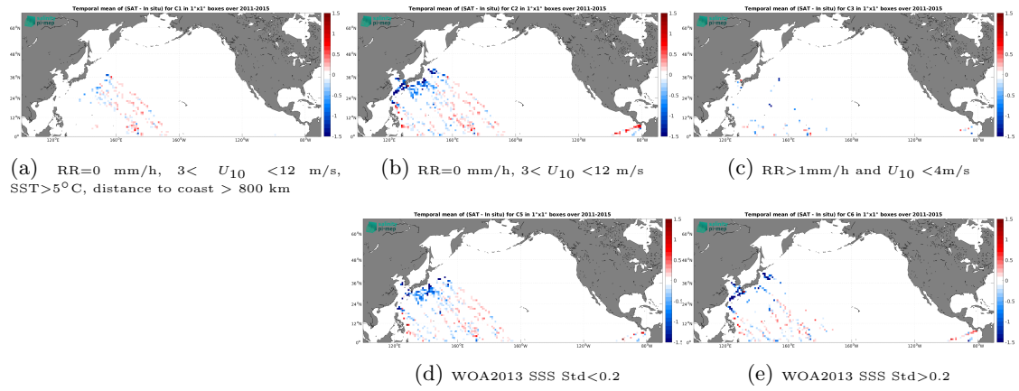
Figure 14: Temporal mean gridded over spatial boxes of size 1^\circ \times 1^\circ of \Delta SSS (Aquarius SSS L2 OR v5 (NASA-GSFC) - TSG (LEGOS-DM)) for 5 different subdatasets corresponding to: RR=0 mm/h, 3 < U_{10} < 12 m/s, SST > 5^\circ C , distance to coast > 800 km (a), RR=0 mm/h, 3 < U_{10} < 12 m/s (b), RR > 1 mm/h and U_{10} < 4 m/s (c), WOA2013 SSS Std < 0.2 (d), WOA2013 SSS Std > 0.2 (e).
