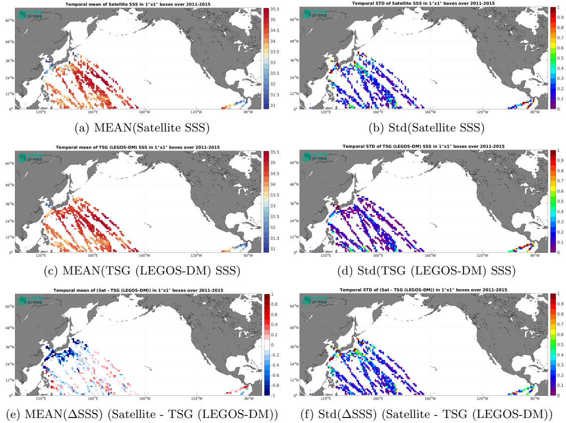
Figure 7: Temporal mean (left) and Std (right) of SSS from Aquarius SSS L2 OR v5 (NASA-GSFC) (top), TSG (LEGOS-DM) (middle), and of \Delta SSS (Satellite - TSG (LEGOS-DM)). Only match-up pairs are used to generate these maps.
