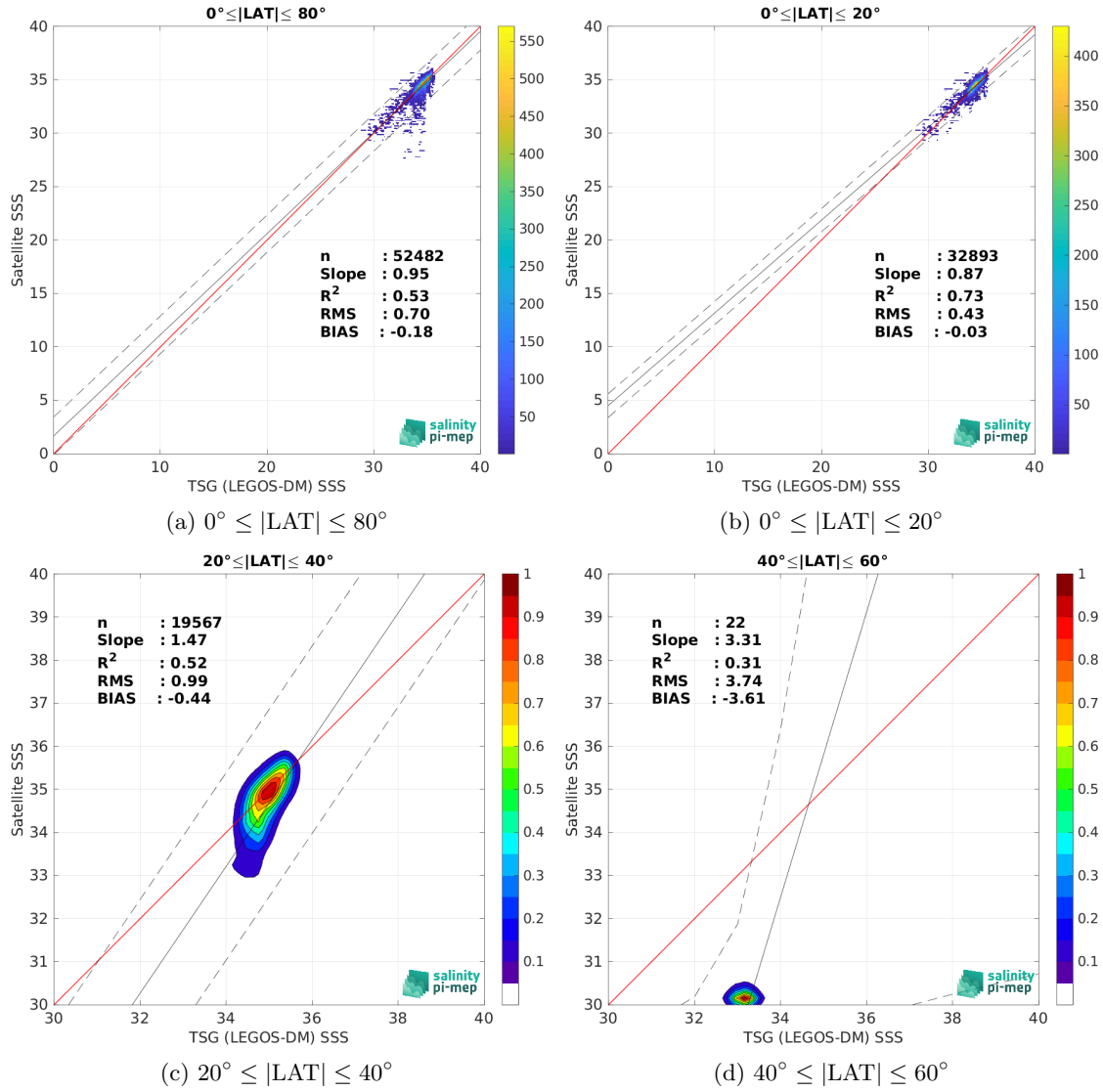
Figure 10: Contour maps of the concentration of Aquarius SSS L2 OR v5 (NASA-GSFC) SSS (y-axis) versus TSG (LEGOS-DM) SSS (x-axis) at match-up pairs for different latitude bands. For each plot, the red line shows x=y . The black thin and dashed lines indicate a linear fit through the data cloud and the \pm 95\% confidence levels, respectively. The number match-up pairs n , the slope and R^2 coefficient of the linear fit, the root mean square (RMS) and the mean bias between satellite and in situ data are indicated for each latitude band in each plots.
