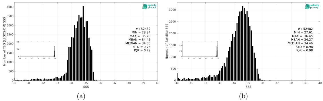
Figure 3: Histograms of SSS from TSG (LEGOS-DM) (a) and Aquarius SSS L2 OR v5 (NASA-GSFC) (b) considering all match-up pairs per bins of 0.1 over the North Pacific Ocean Pi-MEP region and for the full satellite product period.
