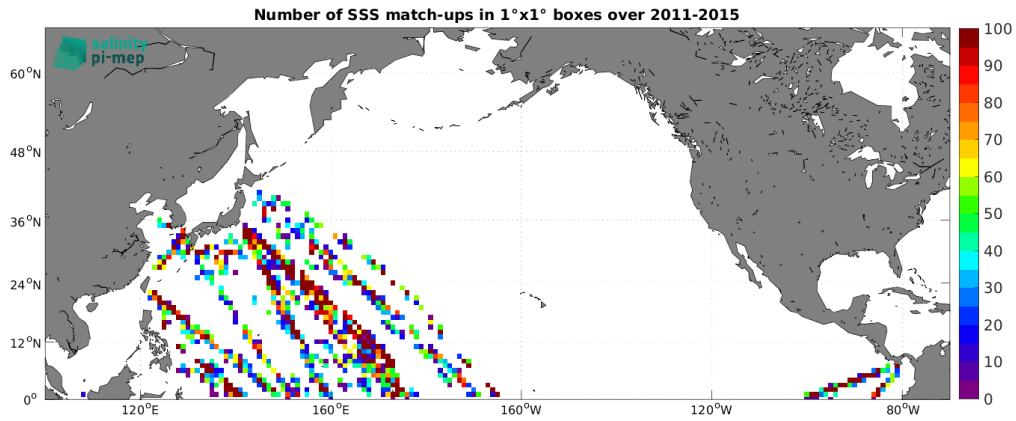
Figure 5: Number of SSS match-ups between TSG (LEGOS-DM) SSS and the Aquarius SSS L2 OR v5 (NASA-GSFC) SSS product for the North Pacific Ocean Pi-MEP region over 1^\circ \times 1^\circ boxes and for the full satellite product period.
