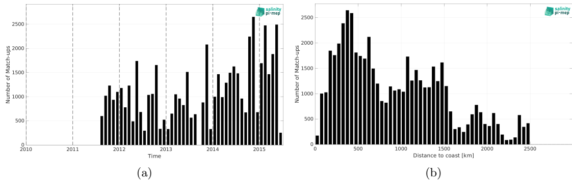
Figure 2: Number of match-ups between TSG (LEGOS-DM) and Aquarius SSS L2 OR v5 (NASA-GSFC) SSS as a function of time (a) and as function of the distance to coast (b) over the North Pacific Ocean Pi-MEP region and for the full satellite product period.
