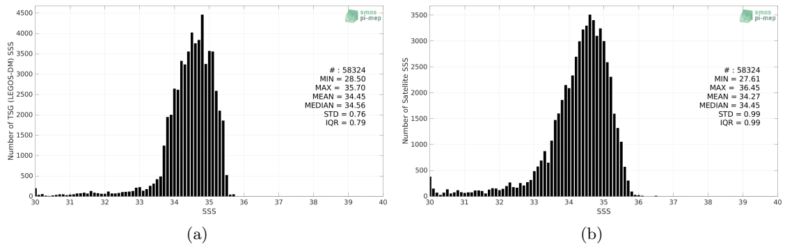
Figure 2: Histograms of SSS from TSG (LEGOS-DM) (a) and Aquarius SSS L2 OR v5 (NASA-GSFC) (b) considering all match-up pairs per bins of 0.1 over the North Pacific Ocean Pi-MEP region and for the full satellite product period.
