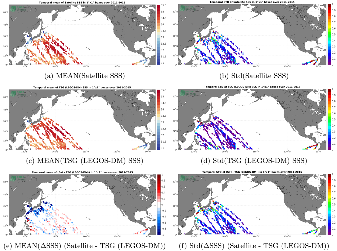
Figure 6: Temporal mean (left) and Std (right) of SSS from Aquarius SSS L2 OR v5 (NASA-GSFC) (top), TSG (LEGOS-DM) (middle), and of \Delta SSS (Satellite - TSG (LEGOS-DM)). Only match-up pairs are used to generate these maps.
