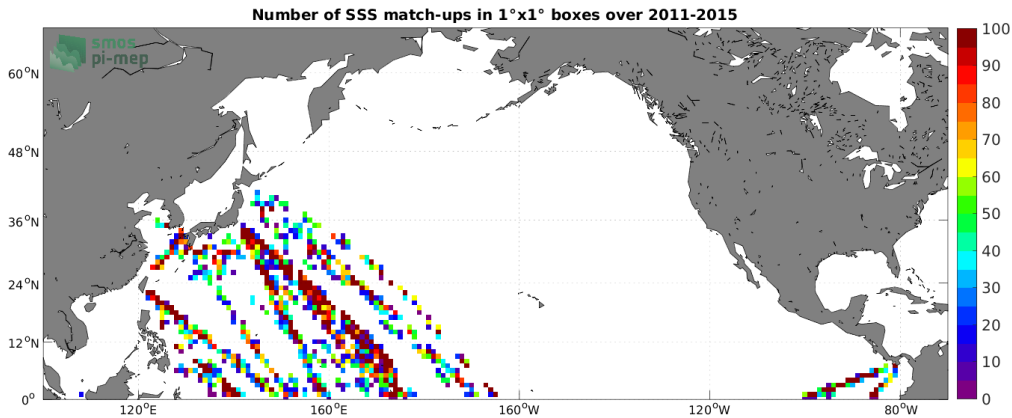
Figure 4: Number of SSS match-ups between TSG (LEGOS-DM) SSS and the Aquarius SSS L2 OR v5 (NASA-GSFC) SSS product for the North Pacific Ocean Pi-MEP region over 1^\circ \times 1^\circ boxes and for the full satellite product period.
