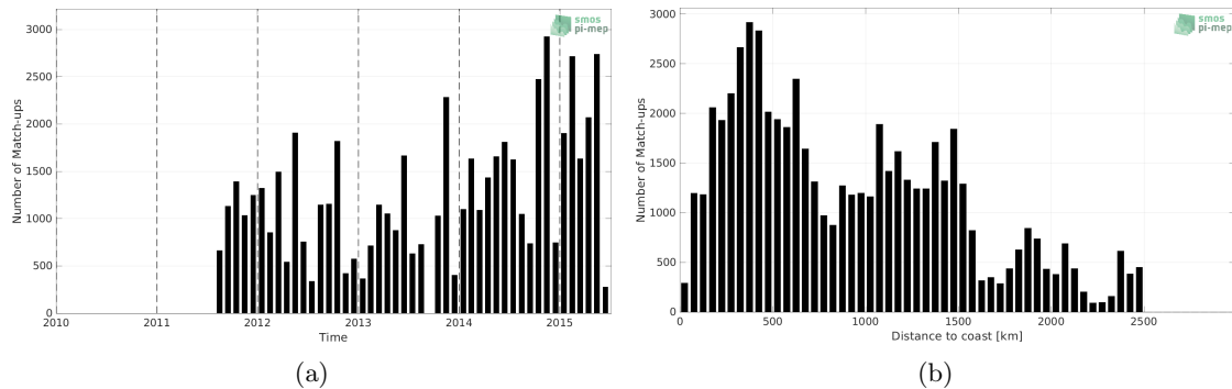
Figure 1: Number of match-ups between TSG (LEGOS-DM) and Aquarius SSS L2 OR v5 (NASA-GSFC) SSS as a function of time (a) and as function of the distance to coast (b) over the North Pacific Ocean Pi-MEP region and for the full satellite product period.
