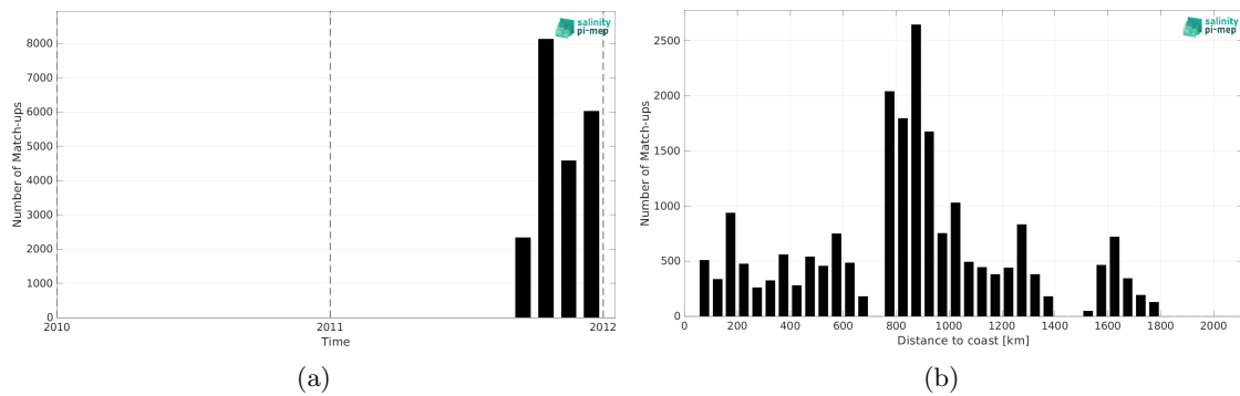
Figure 2: Number of match-ups between TSG (GOSUD-Sailing-ship) and Aquarius SSS L2 OR v5 (NASA-GSFC) SSS as a function of time (a) and as function of the distance to coast (b) over the North Pacific Ocean Pi-MEP region and for the full satellite product period.
