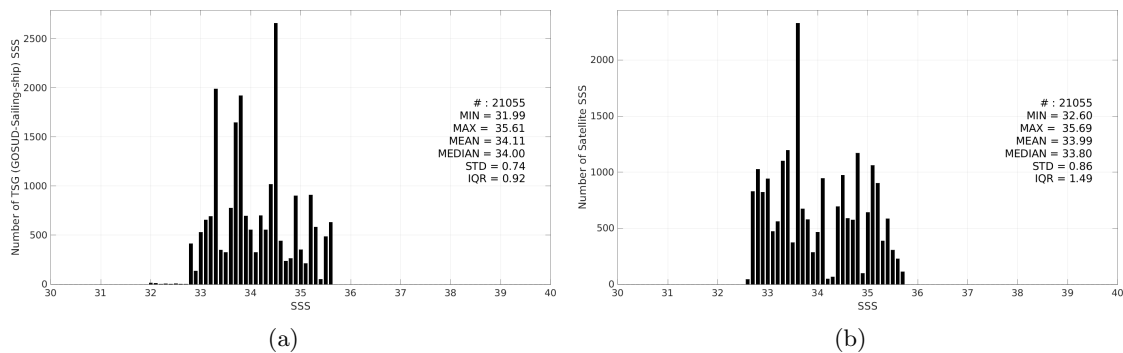
Figure 3: Histograms of SSS from TSG (GOSUD-Sailing-ship) (a) and Aquarius SSS L2 OR v5 (NASA-GSFC) (b) considering all match-up pairs per bins of 0.1 over the North Pacific Ocean Pi-MEP region and for the full satellite product period.
