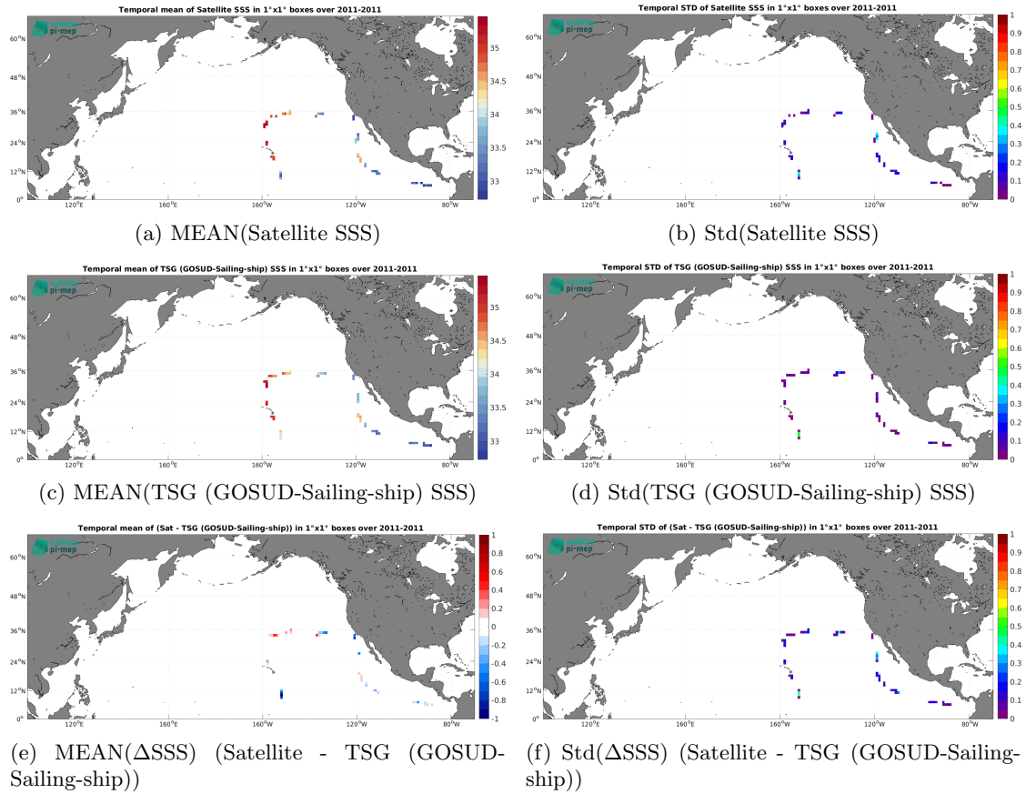
Figure 7: Temporal mean (left) and Std (right) of SSS from Aquarius SSS L2 OR v5 (NASA-GSFC) (top), TSG (GOSUD-Sailing-ship) (middle), and of \Delta SSS (Satellite - TSG (GOSUD-Sailing-ship)). Only match-up pairs are used to generate these maps.
