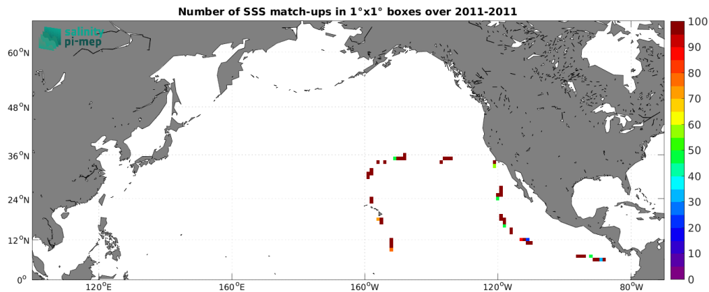
Figure 5: Number of SSS match-ups between TSG (GOSUD-Sailing-ship) SSS and the Aquarius SSS L2 OR v5 (NASA-GSFC) SSS product for the North Pacific Ocean Pi-MEP region over 1^\circ \times 1^\circ boxes and for the full satellite product period.
