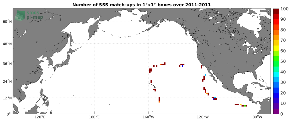
Figure 4: Number of SSS match-ups between TSG (GOSUD-Sailing-ship) SSS and the Aquarius SSS L2 OR v5 (NASA-GSFC) SSS product for the North Pacific Ocean Pi-MEP region over 1^\circ \times 1^\circ boxes and for the full satellite product period.
