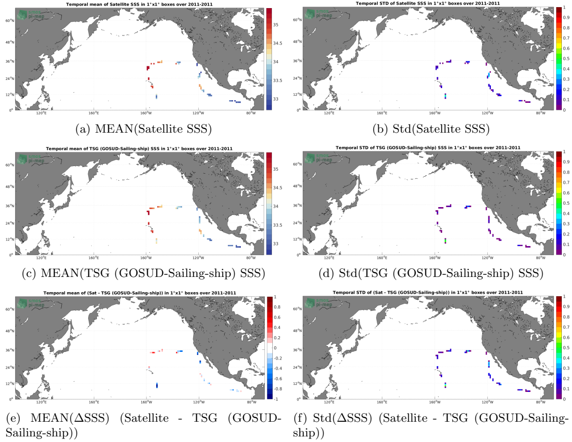
Figure 6: Temporal mean (left) and Std (right) of SSS from Aquarius SSS L2 OR v5 (NASA-GSFC) (top), TSG (GOSUD-Sailing-ship) (middle), and of \Delta SSS (Satellite - TSG (GOSUD-Sailing-ship)). Only match-up pairs are used to generate these maps.
