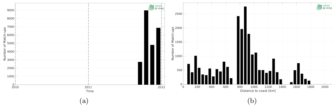
Figure 1: Number of match-ups between TSG (GOSUD-Sailing-ship) and Aquarius SSS L2 OR v5 (NASA-GSFC) SSS as a function of time (a) and as function of the distance to coast (b) over the North Pacific Ocean Pi-MEP region and for the full satellite product period.
