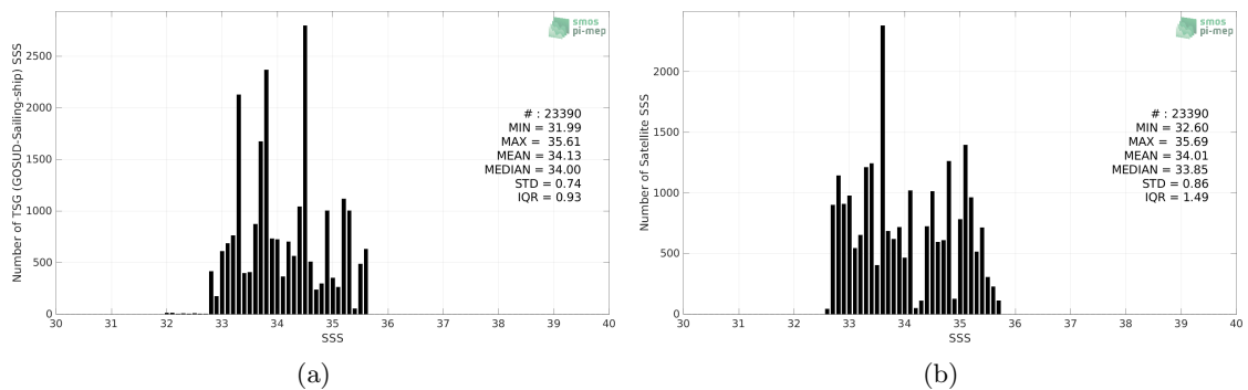
Figure 2: Histograms of SSS from TSG (GOSUD-Sailing-ship) (a) and Aquarius SSS L2 OR v5 (NASA-GSFC) (b) considering all match-up pairs per bins of 0.1 over the North Pacific Ocean Pi-MEP region and for the full satellite product period.
