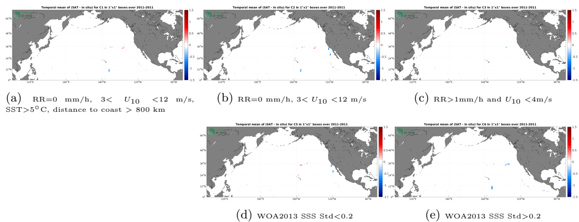
Figure 12: Temporal mean gridded over spatial boxes of size 1^\circ \times 1^\circ of \Delta\text{SSS} (Aquarius SSS L2 OR v5 (NASA-GSFC) - TSG (GOSUD-Sailing-ship)) for 5 different subdatasets corresponding to: RR=0 mm/h, 3 < U_{10} < 12 m/s, SST > 5^\circ\text{C} , distance to coast > 800 km (a), RR=0 mm/h, 3 < U_{10} < 12 m/s (b), RR > 1 mm/h and U_{10} < 4 m/s (c), WOA2013 SSS Std < 0.2 (d), WOA2013 SSS Std > 0.2 (e).
