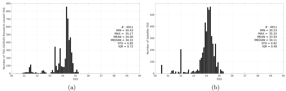
Figure 3: Histograms of SSS from TSG (GOSUD-Research-vessel) (a) and Aquarius SSS L2 OR v5 (NASA-GSFC) (b) considering all match-up pairs per bins of 0.1 over the North Pacific Ocean Pi-MEP region and for the full satellite product period.
