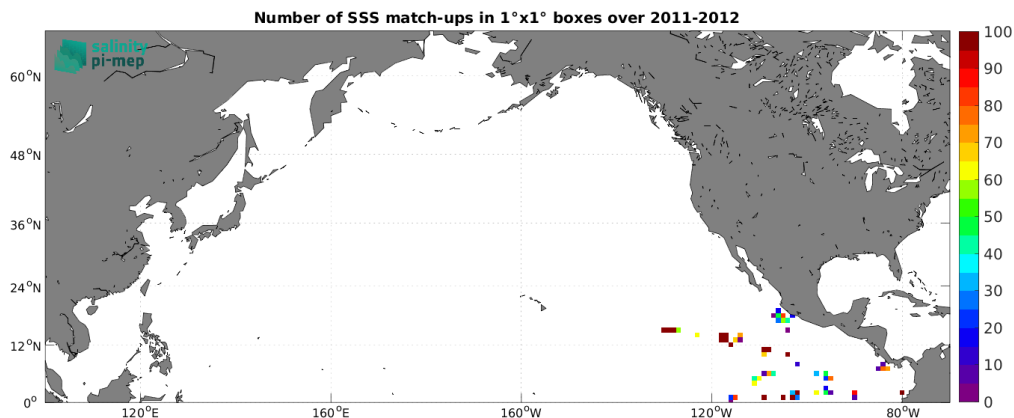
Figure 5: Number of SSS match-ups between TSG (GOSUD-Research-vessel) SSS and the Aquarius SSS L2 OR v5 (NASA-GSFC) SSS product for the North Pacific Ocean Pi-MEP region over 1^\circ \times 1^\circ boxes and for the full satellite product period.
