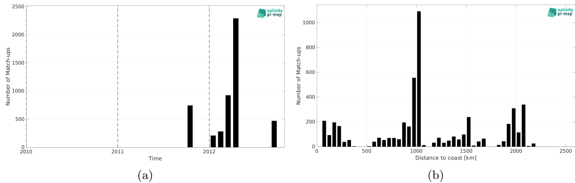
Figure 2: Number of match-ups between TSG (GOSUD-Research-vessel) and Aquarius SSS L2 OR v5 (NASA-GSFC) SSS as a function of time (a) and as function of the distance to coast (b) over the North Pacific Ocean Pi-MEP region and for the full satellite product period.
