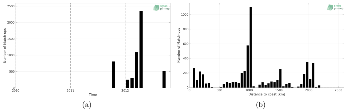
Figure 1: Number of match-ups between TSG (GOSUD-Research-vessel) and Aquarius SSS L2 OR v5 (NASA-GSFC) SSS as a function of time (a) and as function of the distance to coast (b) over the North Pacific Ocean Pi-MEP region and for the full satellite product period.
