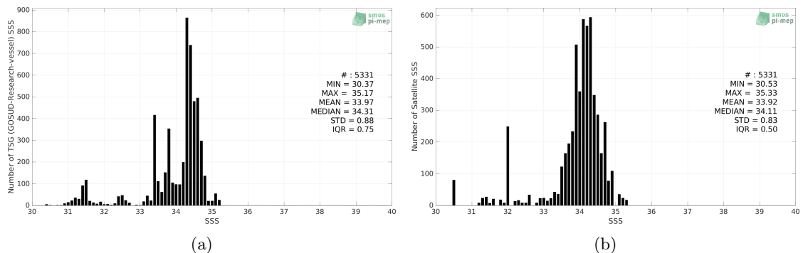
Figure 2: Histograms of SSS from TSG (GOSUD-Research-vessel) (a) and Aquarius SSS L2 OR v5 (NASA-GSFC) (b) considering all match-up pairs per bins of 0.1 over the North Pacific Ocean Pi-MEP region and for the full satellite product period.
