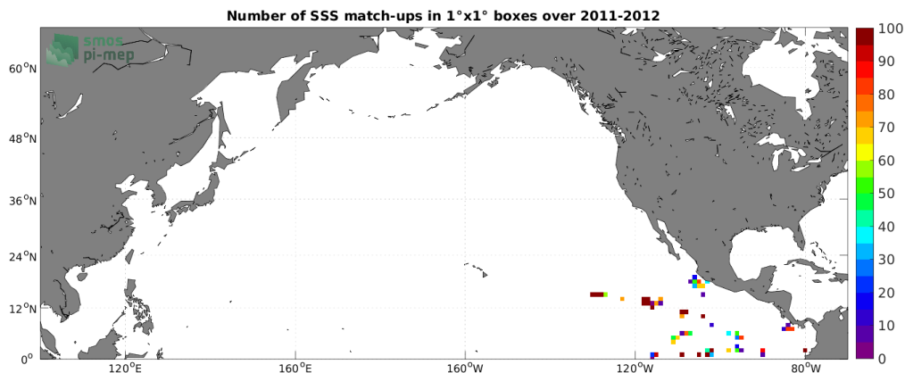
Figure 4: Number of SSS match-ups between TSG (GOSUD-Research-vessel) SSS and the Aquarius SSS L2 OR v5 (NASA-GSFC) SSS product for the North Pacific Ocean Pi-MEP region over 1^\circ \times 1^\circ boxes and for the full satellite product period.
