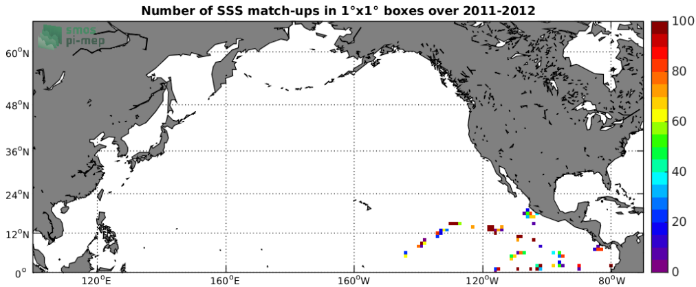
Figure 4: Number of SSS match-ups between TSG-GOSUD-Research-vessel SSS and the Aquarius-L2-OR-V5 SSS product for the North Pacific Ocean Pi-MEP region over 1^\circ \times 1^\circ boxes and for the full satellite product period.
