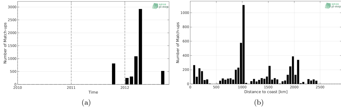
Figure 1: Number of match-ups between TSG-GOSUD-Research-vessel and Aquarius-L2-OR-V5 SSS as a function of time (a) and as function of the distance to coast (b) over the North Pacific Ocean Pi-MEP region and for the full satellite product period.
