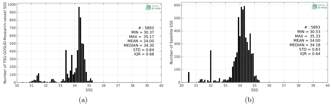
Figure 2: Histograms of SSS from TSG-GOSUD-Research-vessel (a) and Aquarius-L2-OR-V5 (b) considering all match-up pairs per bins of 0.1 over the North Pacific Ocean Pi-MEP region and for the full satellite product period.
