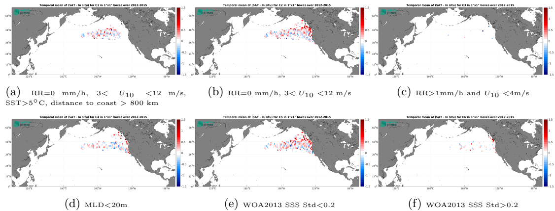
Figure 14: Temporal mean gridded over spatial boxes of size 1^\circ \times 1^\circ of \Delta SSS (Aquarius SSS L2 OR v5 (NASA-GSFC) - Marine mammals) for 6 different subdatasets corresponding to: RR=0 mm/h, 3 < U_{10} < 12 m/s, SST > 5°C, distance to coast > 800 km (a), RR=0 mm/h, 3 < U_{10} < 12 m/s (b), RR > 1 mm/h and U_{10} < 4 m/s (c), MLD < 20 m (d), WOA2013 SSS Std < 0.2 (e), WOA2013 SSS Std > 0.2 (f).
