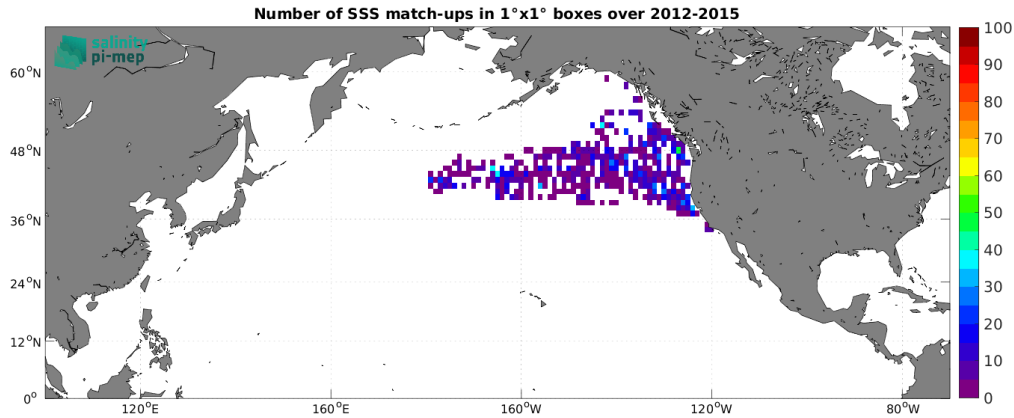
Figure 5: Number of SSS match-ups between Marine mammals SSS and the Aquarius SSS L2 OR v5 (NASA-GSFC) SSS product for the North Pacific Ocean Pi-MEP region over 1^\circ \times 1^\circ boxes and for the full satellite product period.
