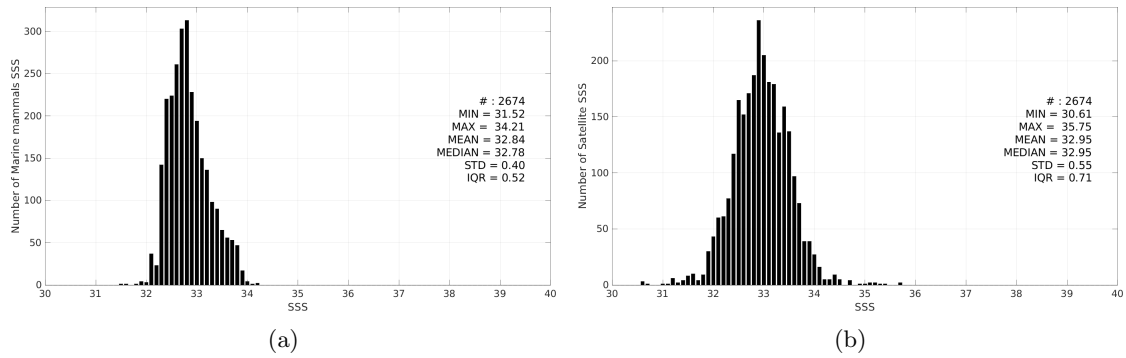
Figure 3: Histograms of SSS from Marine mammals (a) and Aquarius SSS L2 OR v5 (NASA-GSFC) (b) considering all match-up pairs per bins of 0.1 over the North Pacific Ocean Pi-MEP region and for the full satellite product period.
