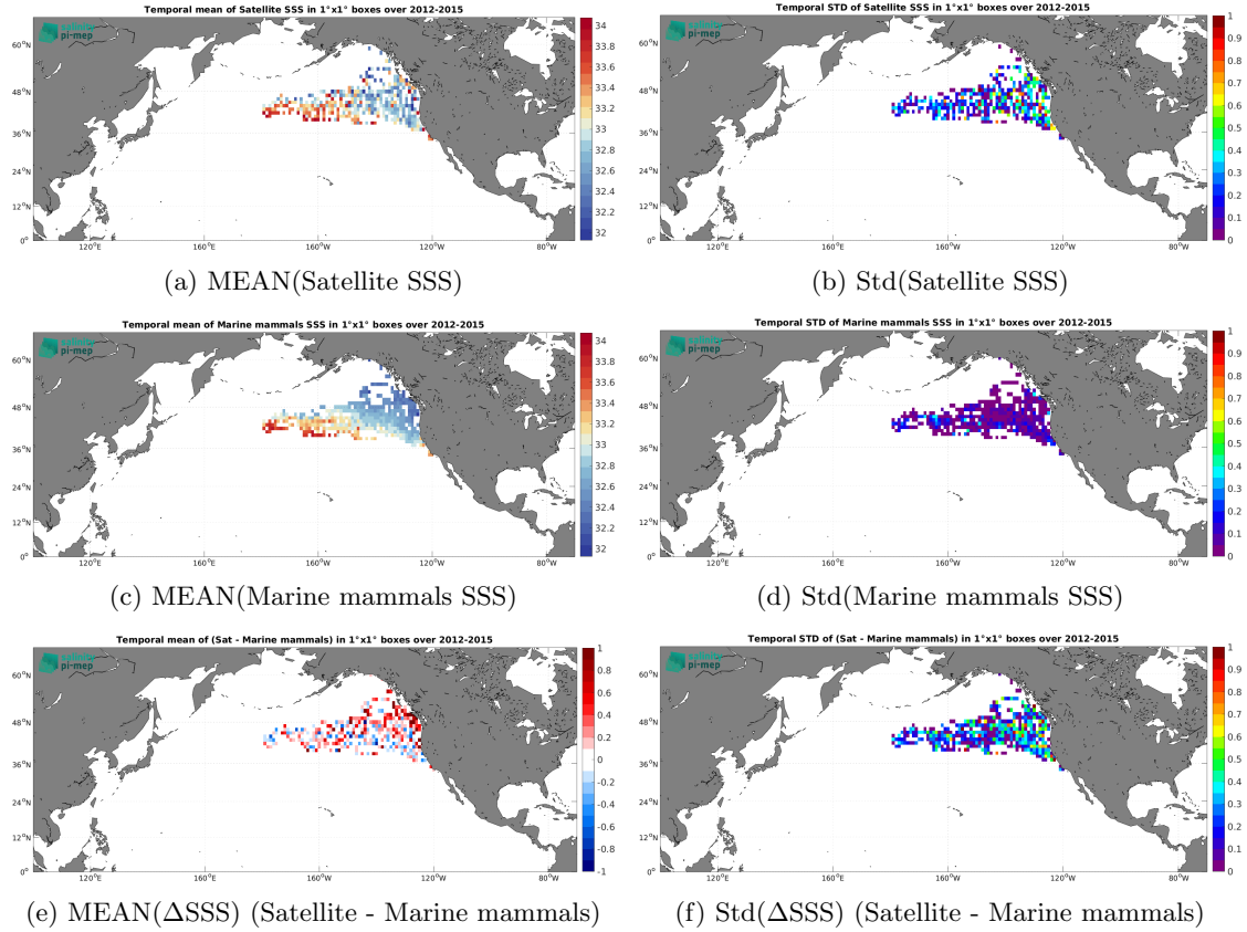
Figure 7: Temporal mean (left) and Std (right) of SSS from Aquarius SSS L2 OR v5 (NASA-GSFC) (top), Marine mammals (middle), and of \Delta SSS (Satellite - Marine mammals). Only match-up pairs are used to generate these maps.
