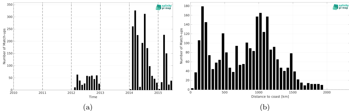
Figure 2: Number of match-ups between Marine mammals and Aquarius SSS L2 OR v5 (NASA-GSFC) SSS as a function of time (a) and as function of the distance to coast (b) over the North Pacific Ocean Pi-MEP region and for the full satellite product period.
