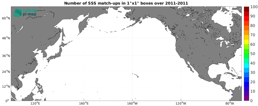
Figure 4: Number of SSS match-ups between Surface drifters SSS and the Aquarius SSS L2 OR v5 (NASA-GSFC) SSS product for the North Pacific Ocean Pi-MEP region over 1^\circ \times 1^\circ boxes and for the full satellite product period.
