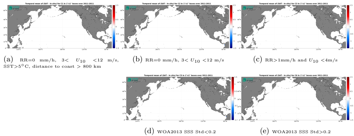
Figure 13: Temporal mean gridded over spatial boxes of size 1^\circ \times 1^\circ of \Delta SSS (Aquarius SSS L2 OR v5 (NASA-GSFC) - Surface drifters) for 5 different subdatasets corresponding to:RR=0 mm/h, 3 < U_{10} < 12 m/s, SST >5^\circ C, distance to coast > 800 km (a), RR=0 mm/h, 3 < U_{10} < 12 m/s (b), RR >1 mm/h and U_{10} < 4 m/s (c), WOA2013 SSS Std <0.2 (d), WOA2013 SSS Std >0.2 (e).
