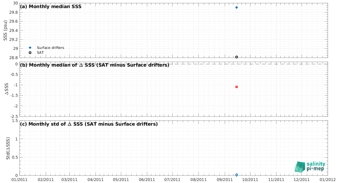
Figure 7: Time series of the monthly median SSS (top), median of \Delta\text{SSS} (Satellite - Surface drifters) and Std of \Delta\text{SSS} (Satellite - Surface drifters) over the North Pacific Ocean Pi-MEP region considering all match-ups collected by the Pi-MEP.
