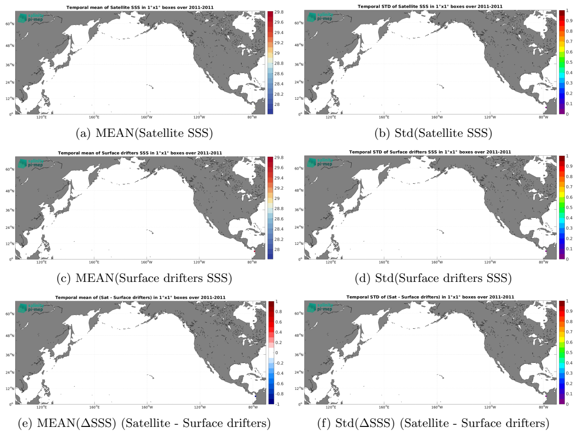
Figure 6: Temporal mean (left) and Std (right) of SSS from Aquarius SSS L2 OR v5 (NASA-GSFC) (top), Surface drifters (middle), and of \Delta SSS (Satellite - Surface drifters). Only match-up pairs are used to generate these maps.
