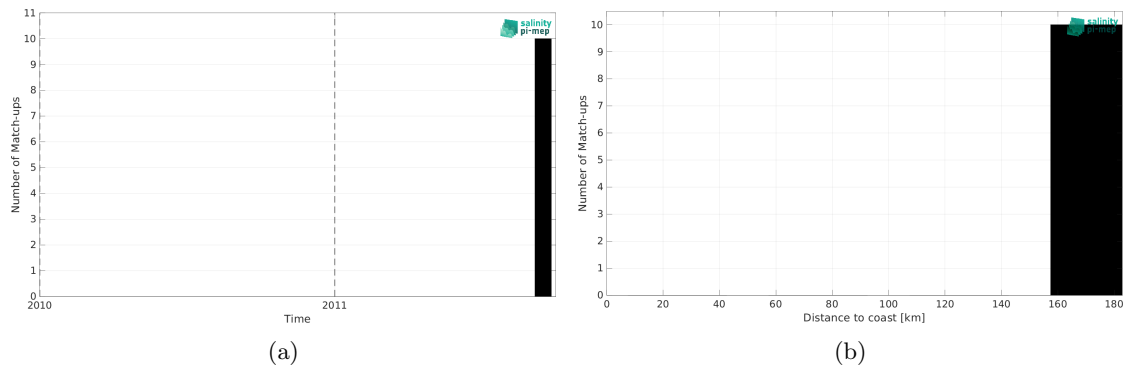
Figure 2: Number of match-ups between Surface drifters and Aquarius SSS L2 OR v5 (NASA-GSFC) SSS as a function of time (a) and as function of the distance to coast (b) over the North Pacific Ocean Pi-MEP region and for the full satellite product period.
