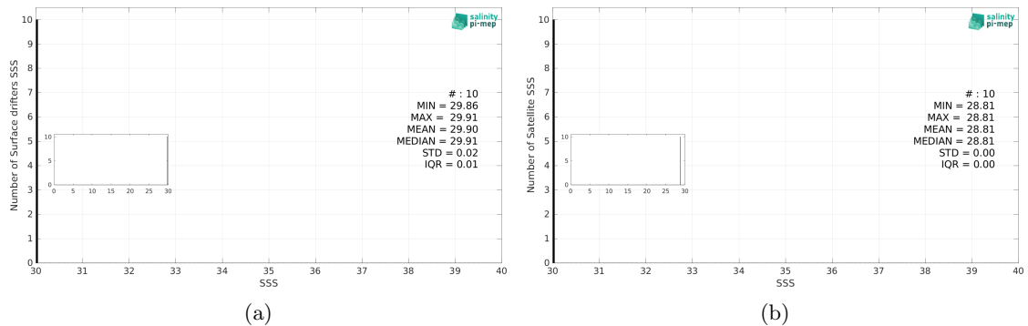
Figure 3: Histograms of SSS from Surface drifters (a) and Aquarius SSS L2 OR v5 (NASA-GSFC) (b) considering all match-up pairs per bins of 0.1 over the North Pacific Ocean Pi-MEP region and for the full satellite product period.
