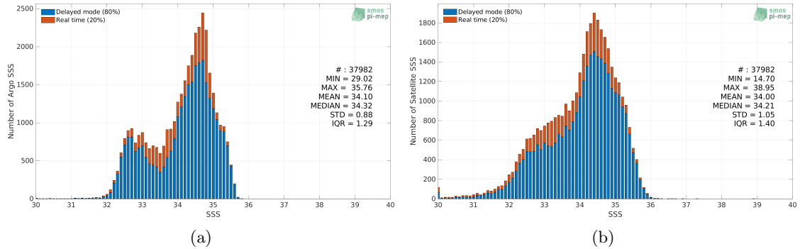
Figure 2: Histograms of SSS from Argo (a) and Aquarius SSS L2 OR v5 (NASA-GSFC) (b) considering all match-up pairs per bins of 0.1 over the North Pacific Ocean Pi-MEP region and for the full satellite product period.
