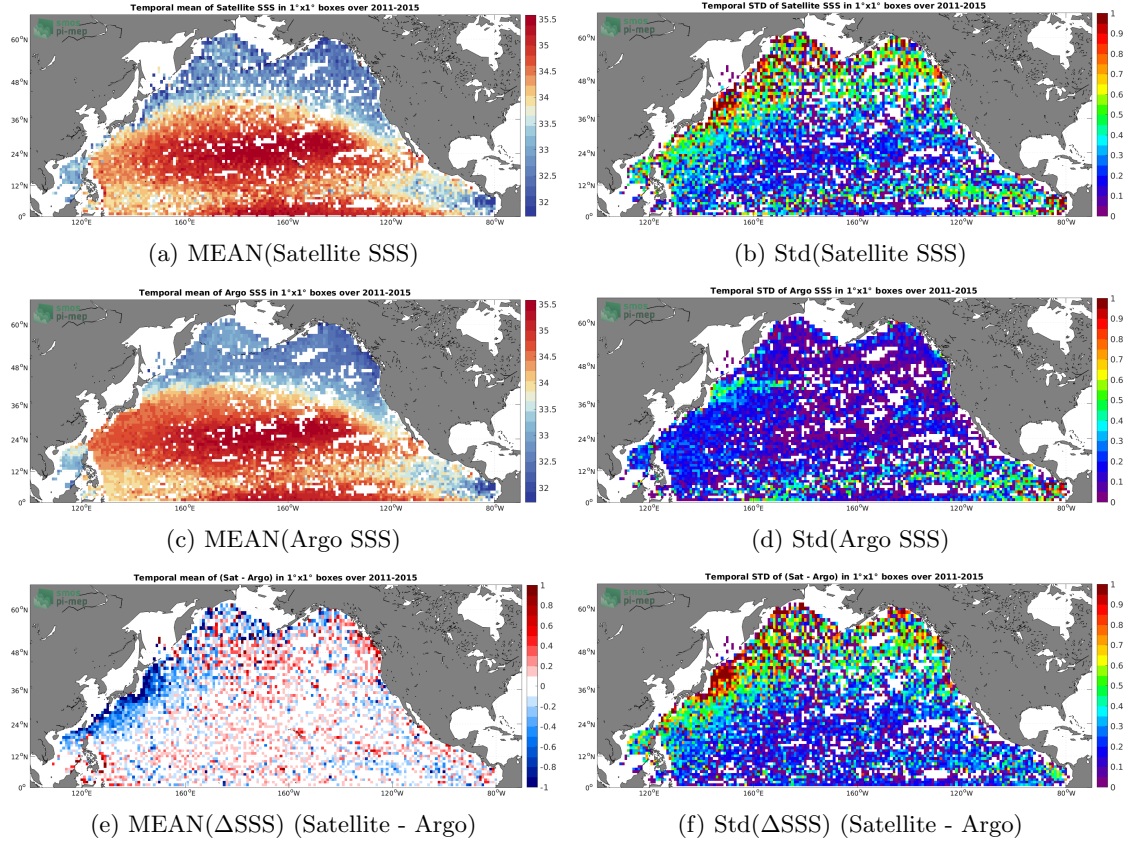
Figure 6: Temporal mean (left) and Std (right) of SSS from Aquarius SSS L2 OR v5 (NASA-GSFC) (top), Argo (middle), and of \Delta\text{SSS} (Satellite - Argo). Only match-up pairs are used to generate these maps.
