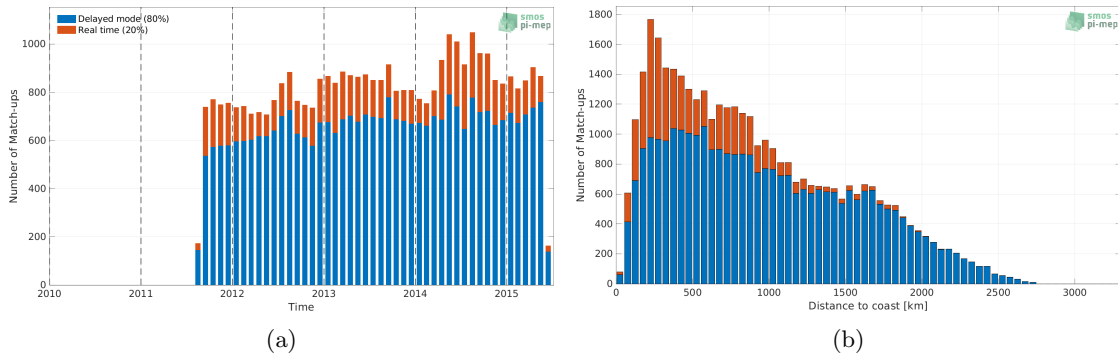
Figure 1: Number of match-ups between Argo and Aquarius SSS L2 OR v5 (NASA-GSFC) SSS as a function of time (a) and as function of the distance to coast (b) over the North Pacific Ocean Pi-MEP region and for the full satellite product period.
