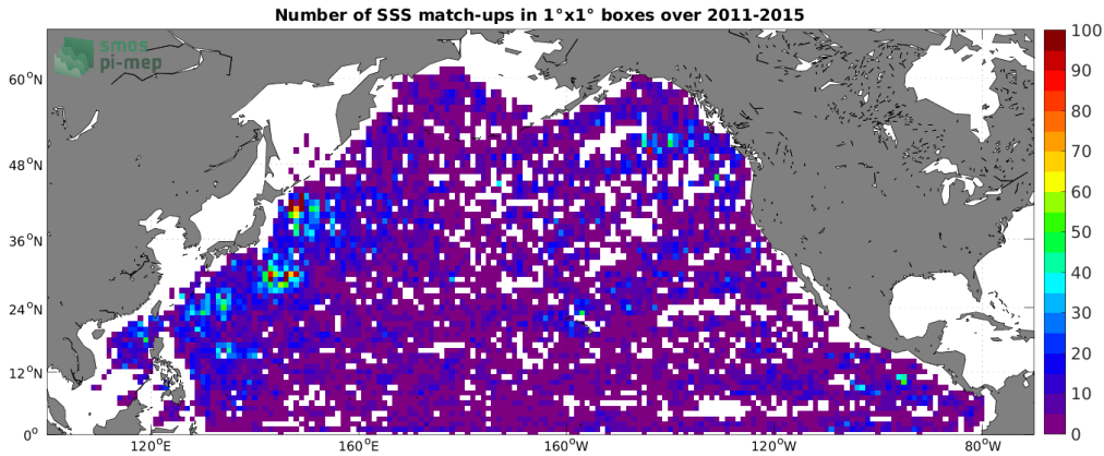
Figure 4: Number of SSS match-ups between Argo SSS and the Aquarius SSS L2 OR v5 (NASA-GSFC) SSS product for the North Pacific Ocean Pi-MEP region over 1^\circ \times 1^\circ boxes and for the full satellite product period.
