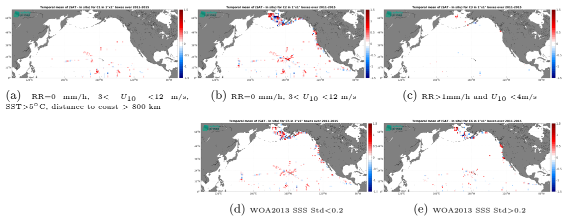
Figure 14: Temporal mean gridded over spatial boxes of size 1^\circ \times 1^\circ of \Delta\text{SSS} (Aquarius SSS L2 CAP v5 (JPL) - TSG (SAMOS)) for 5 different subdatasets corresponding to:RR=0 mm/h, 3 < U_{10} < 12 m/s, SST > 5°C, distance to coast > 800 km (a), RR=0 mm/h, 3 < U_{10} < 12 m/s (b), RR > 1mm/h and U_{10} < 4 m/s (c), WOA2013 SSS Std < 0.2 (d), WOA2013 SSS Std > 0.2 (e).
