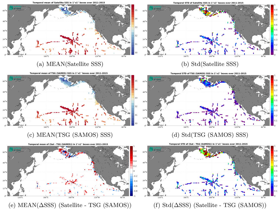
Figure 7: Temporal mean (left) and Std (right) of SSS from Aquarius SSS L2 CAP v5 (JPL) (top), TSG (SAMOS) (middle), and of \Delta SSS (Satellite - TSG (SAMOS)). Only match-up pairs are used to generate these maps.
