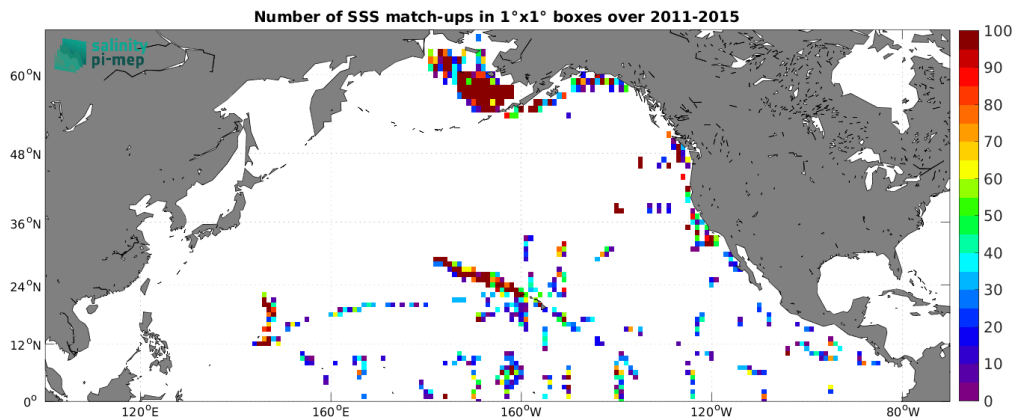
Figure 5: Number of SSS match-ups between TSG (SAMOS) SSS and the Aquarius SSS L2 CAP v5 (JPL) SSS product for the North Pacific Ocean Pi-MEP region over 1^\circ \times 1^\circ boxes and for the full satellite product period.
