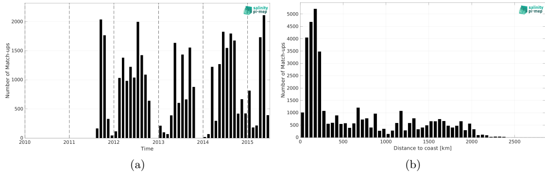
Figure 2: Number of match-ups between TSG (SAMOS) and Aquarius SSS L2 CAP v5 (JPL) SSS as a function of time (a) and as function of the distance to coast (b) over the North Pacific Ocean Pi-MEP region and for the full satellite product period.
