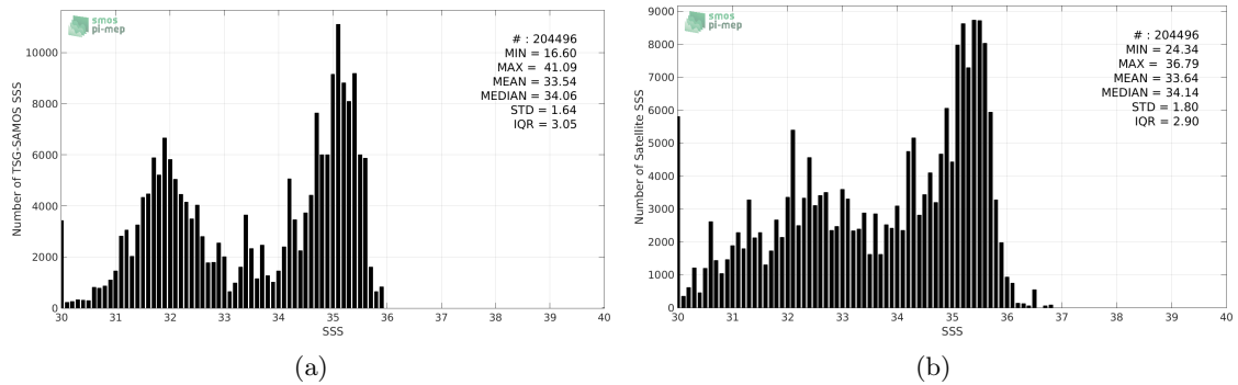
Figure 2: Histograms of SSS from TSG-SAMOS (a) and Aquarius-L2-JPL-V5 (b) considering all match-up pairs per bins of 0.1 over the North Pacific Ocean Pi-MEP region and for the full satellite product period.
