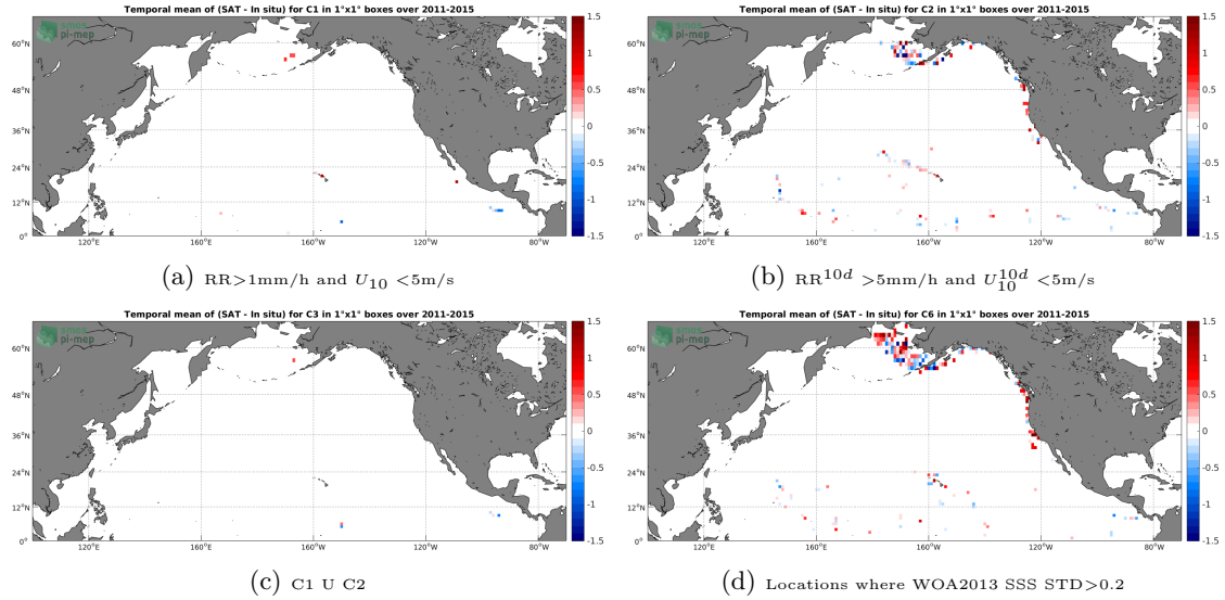
Figure 12: Temporal mean gridded over spatial boxes of size 1^\circ \times 1^\circ of \Delta SSS (Aquarius-L2-JPL-V5 - TSG-SAMOS) for 4 different subdatasets corresponding to: RR > 1\text{mm/h} and U_{10} < 5\text{m/s} (a), RR^{10d} > 5\text{mm/h} and U_{10}^{10d} < 5\text{m/s} (b), C1 U C2 (c), Locations where WOA2013 SSS STD > 0.2 (d).
