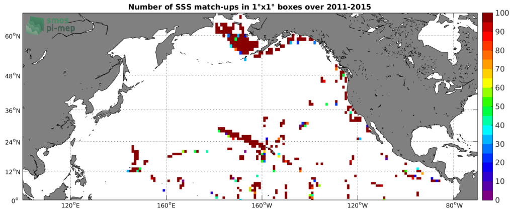
Figure 4: Number of SSS match-ups between TSG-SAMOS SSS and the Aquarius-L2-JPL-V5 SSS product for the North Pacific Ocean Pi-MEP region over 1^\circ \times 1^\circ boxes and for the full satellite product period.
