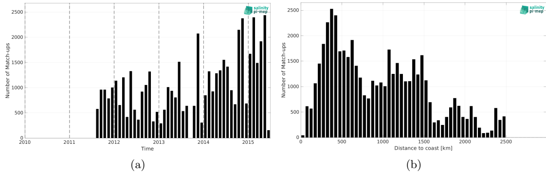
Figure 2: Number of match-ups between TSG (LEGOS-DM) and Aquarius SSS L2 CAP v5 (JPL) SSS as a function of time (a) and as function of the distance to coast (b) over the North Pacific Ocean Pi-MEP region and for the full satellite product period.
