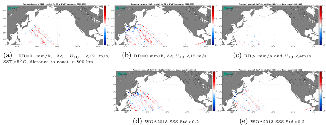
Figure 14: Temporal mean gridded over spatial boxes of size 1^\circ \times 1^\circ of \Delta\text{SSS} (Aquarius SSS L2 CAP v5 (JPL) - TSG (LEGOS-DM)) for 5 different subdatasets corresponding to:RR=0 mm/h, 3 < U_{10} < 12 m/s, SST > 5°C, distance to coast > 800 km (a), RR=0 mm/h, 3 < U_{10} < 12 m/s (b), RR > 1mm/h and U_{10} < 4 m/s (c), WOA2013 SSS Std < 0.2 (d), WOA2013 SSS Std > 0.2 (e).
