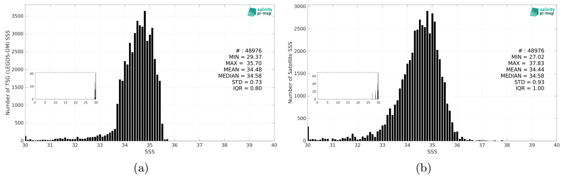
Figure 3: Histograms of SSS from TSG (LEGOS-DM) (a) and Aquarius SSS L2 CAP v5 (JPL) (b) considering all match-up pairs per bins of 0.1 over the North Pacific Ocean Pi-MEP region and for the full satellite product period.
