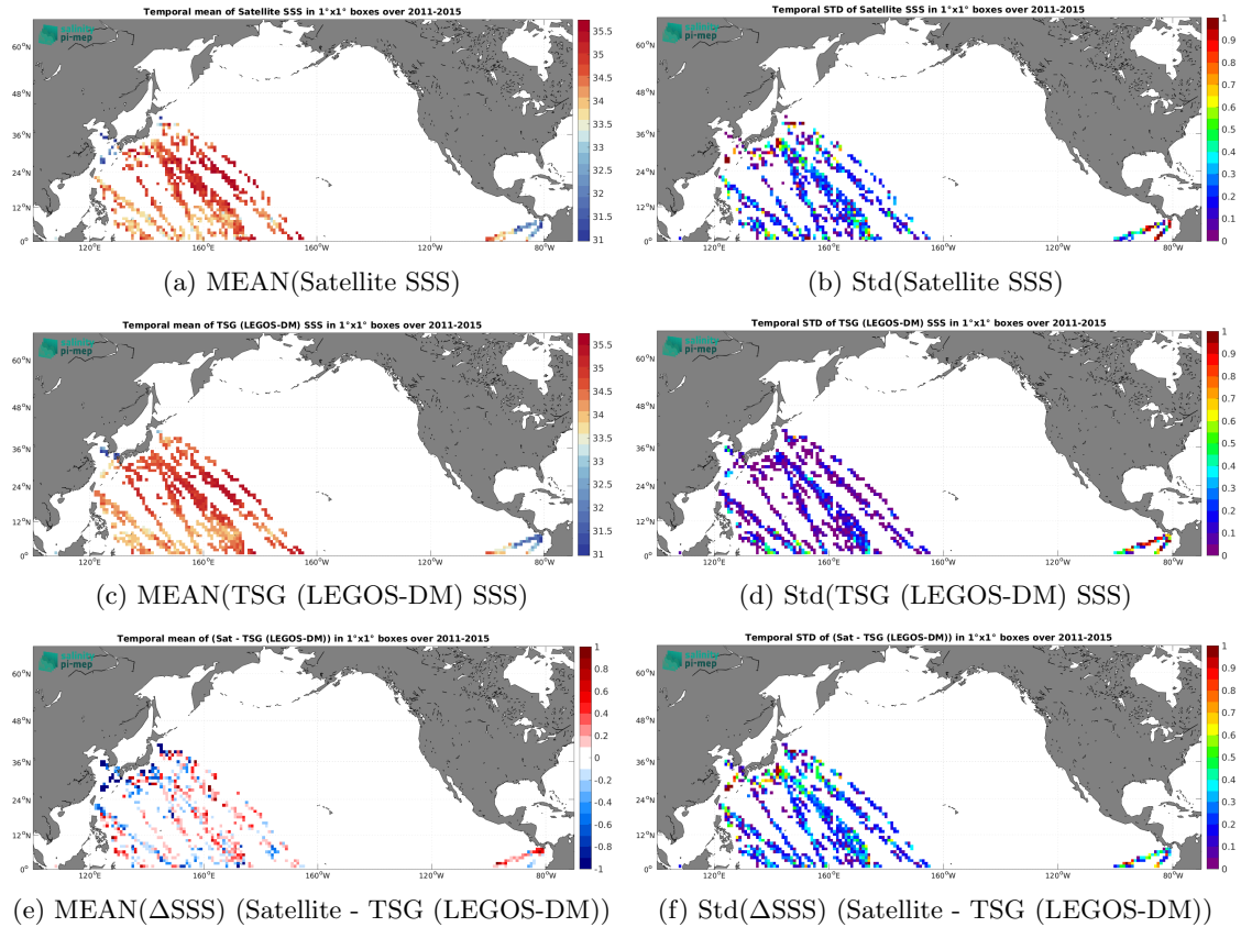
Figure 7: Temporal mean (left) and Std (right) of SSS from Aquarius SSS L2 CAP v5 (JPL) (top), TSG (LEGOS-DM) (middle), and of \Delta SSS (Satellite - TSG (LEGOS-DM)). Only match-up pairs are used to generate these maps.
