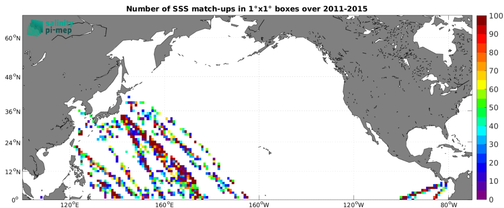
Figure 5: Number of SSS match-ups between TSG (LEGOS-DM) SSS and the Aquarius SSS L2 CAP v5 (JPL) SSS product for the North Pacific Ocean Pi-MEP region over 1^\circ \times 1^\circ boxes and for the full satellite product period.
