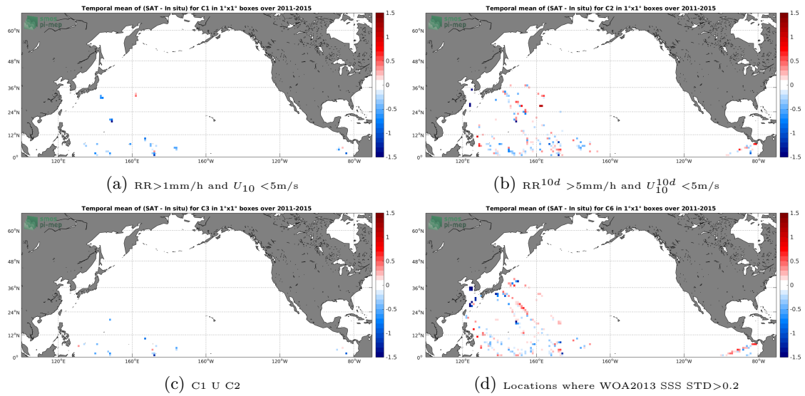
Figure 12: Temporal mean gridded over spatial boxes of size 1^\circ \times 1^\circ of \Delta SSS (Aquarius-L2-JPL-V5 - TSG-LEGOS-DM) for 4 different subdatasets corresponding to: RR > 1\text{mm/h} and U_{10} < 5\text{m/s} (a), RR^{10d} > 5\text{mm/h} and U_{10}^{10d} < 5\text{m/s} (b), C1 U C2 (c), Locations where WOA2013 SSS STD > 0.2 (d).
