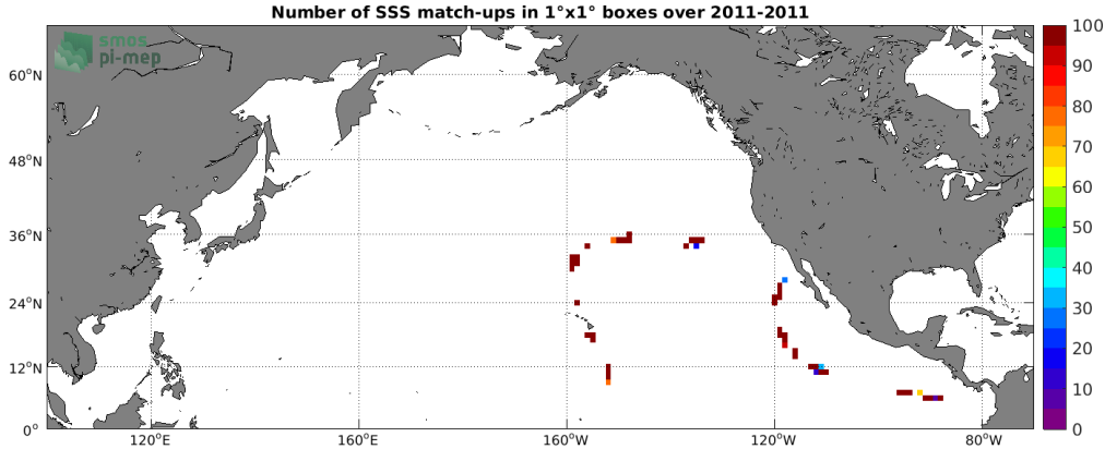
Figure 4: Number of SSS match-ups between TSG (GOSUD-Sailing-ship) SSS and the Aquarius SSS L2 CAP v5 (JPL) SSS product for the North Pacific Ocean Pi-MEP region over 1°x1° boxes and for the full satellite product period.
