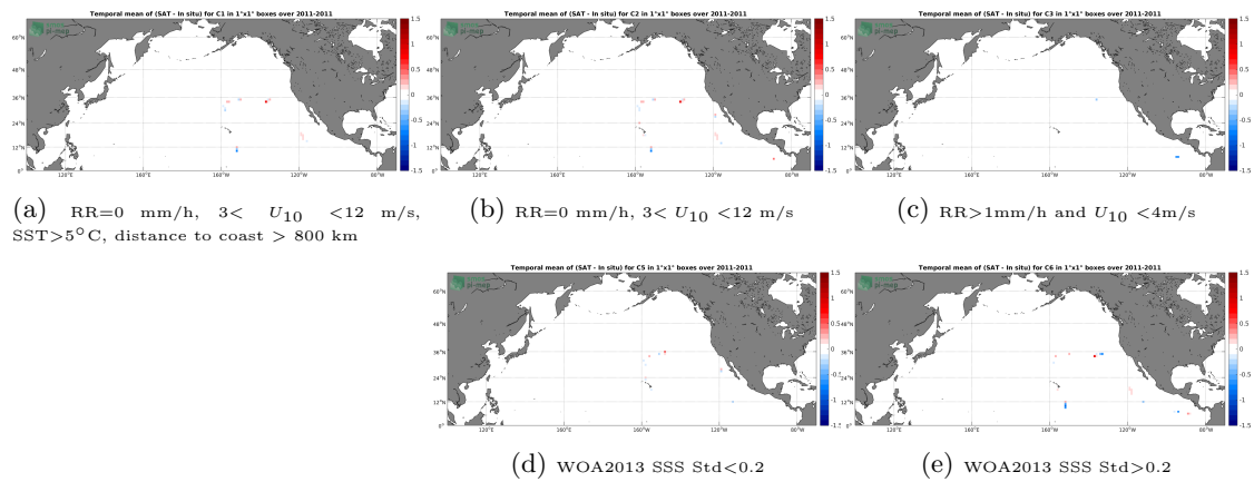
Figure 12: Temporal mean gridded over spatial boxes of size 1^\circ \times 1^\circ of \Delta SSS (Aquarius-L2-JPL-V5 - TSG-GOSUD-Sailing-ship) for 5 different subdatasets corresponding to:RR=0 mm/h, 3 < U_{10} < 12 m/s, SST > 5^\circ\text{C} , distance to coast > 800 km (a), RR=0 mm/h, 3 < U_{10} < 12 m/s (b), RR > 1 mm/h and U_{10} < 4 m/s (c), WOA2013 SSS Std < 0.2 (d), WOA2013 SSS Std > 0.2 (e).
