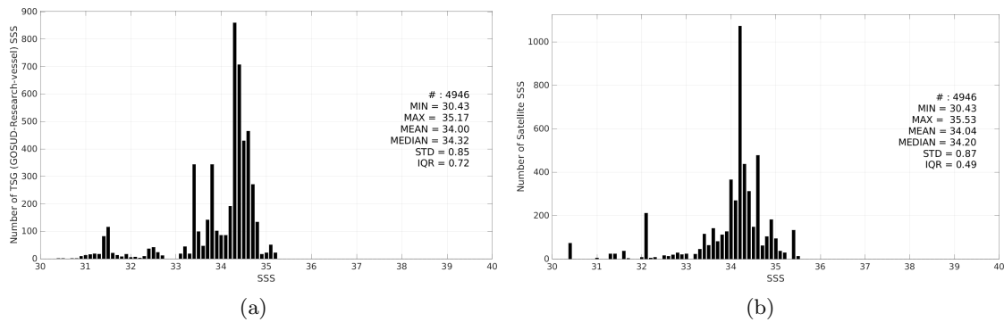
Figure 3: Histograms of SSS from TSG (GOSUD-Research-vessel) (a) and Aquarius SSS L2 CAP v5 (JPL) (b) considering all match-up pairs per bins of 0.1 over the North Pacific Ocean Pi-MEP region and for the full satellite product period.
