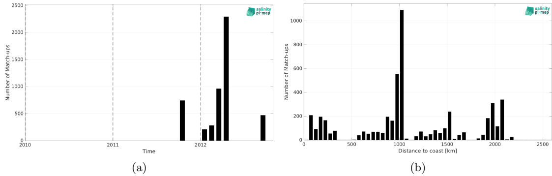
Figure 2: Number of match-ups between TSG (GOSUD-Research-vessel) and Aquarius SSS L2 CAP v5 (JPL) SSS as a function of time (a) and as function of the distance to coast (b) over the North Pacific Ocean Pi-MEP region and for the full satellite product period.
