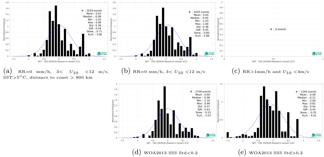
Figure 15: Normalized histogram of \Delta SSS (Aquarius SSS L2 CAP v5 (JPL) - TSG (GOSUD-Research-vessel)) for 5 different subdatasets corresponding to: RR=0 mm/h, 3 < U_{10} < 12 m/s, SST > 5°C, distance to coast > 800 km (a), RR=0 mm/h, 3 < U_{10} < 12 m/s (b), RR > 1mm/h and U_{10} < 4 m/s (c), WOA2013 SSS Std < 0.2 (d), WOA2013 SSS Std > 0.2 (e).
