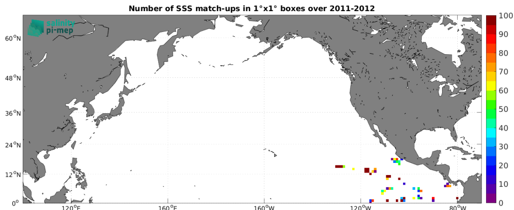
Figure 5: Number of SSS match-ups between TSG (GOSUD-Research-vessel) SSS and the Aquarius SSS L2 CAP v5 (JPL) SSS product for the North Pacific Ocean Pi-MEP region over 1^\circ \times 1^\circ boxes and for the full satellite product period.
