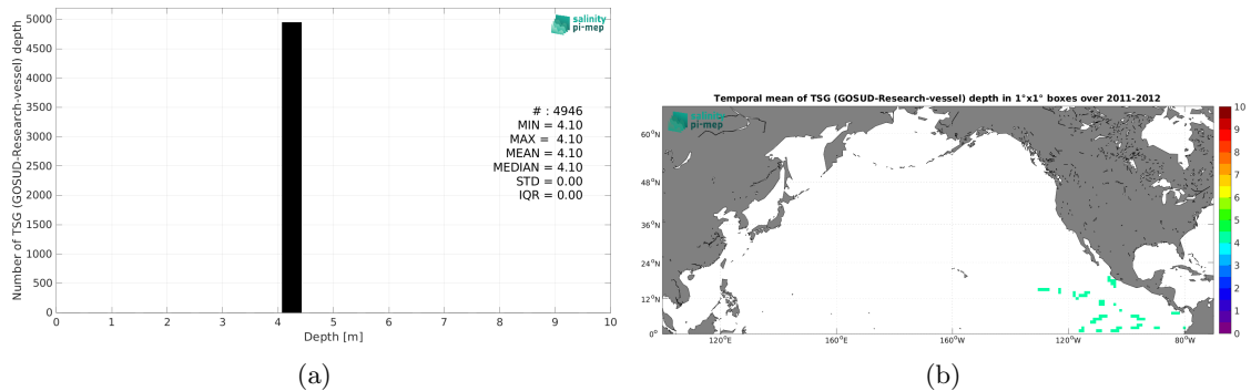
Figure 4: Histograms of the depth of the upper level SSS measurements from TSG (GOSUD-Research-vessel) in the Match-up DataBase for the North Pacific Ocean Pi-MEP region (a) and temporal mean spatial distribution of pressure of the in situ SSS data over 1^\circ \times 1^\circ boxes and for the full satellite product period (b).
