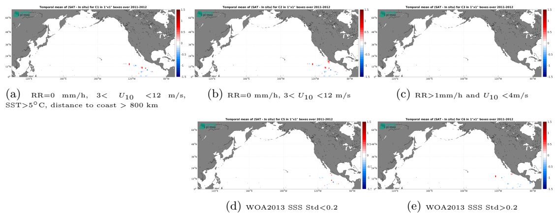
Figure 14: Temporal mean gridded over spatial boxes of size 1^\circ \times 1^\circ of \Delta\text{SSS} (Aquarius SSS L2 CAP v5 (JPL) - TSG (GOSUD-Research-vessel)) for 5 different subdatasets corresponding to:RR=0 mm/h, 3 < U_{10} < 12 m/s, SST >5^\circ\text{C} , distance to coast > 800 km (a), RR=0 mm/h, 3 < U_{10} < 12 m/s (b), RR >1 mm/h and U_{10} < 4 m/s (c), WOA2013 SSS Std <0.2 (d), WOA2013 SSS Std >0.2 (e).
