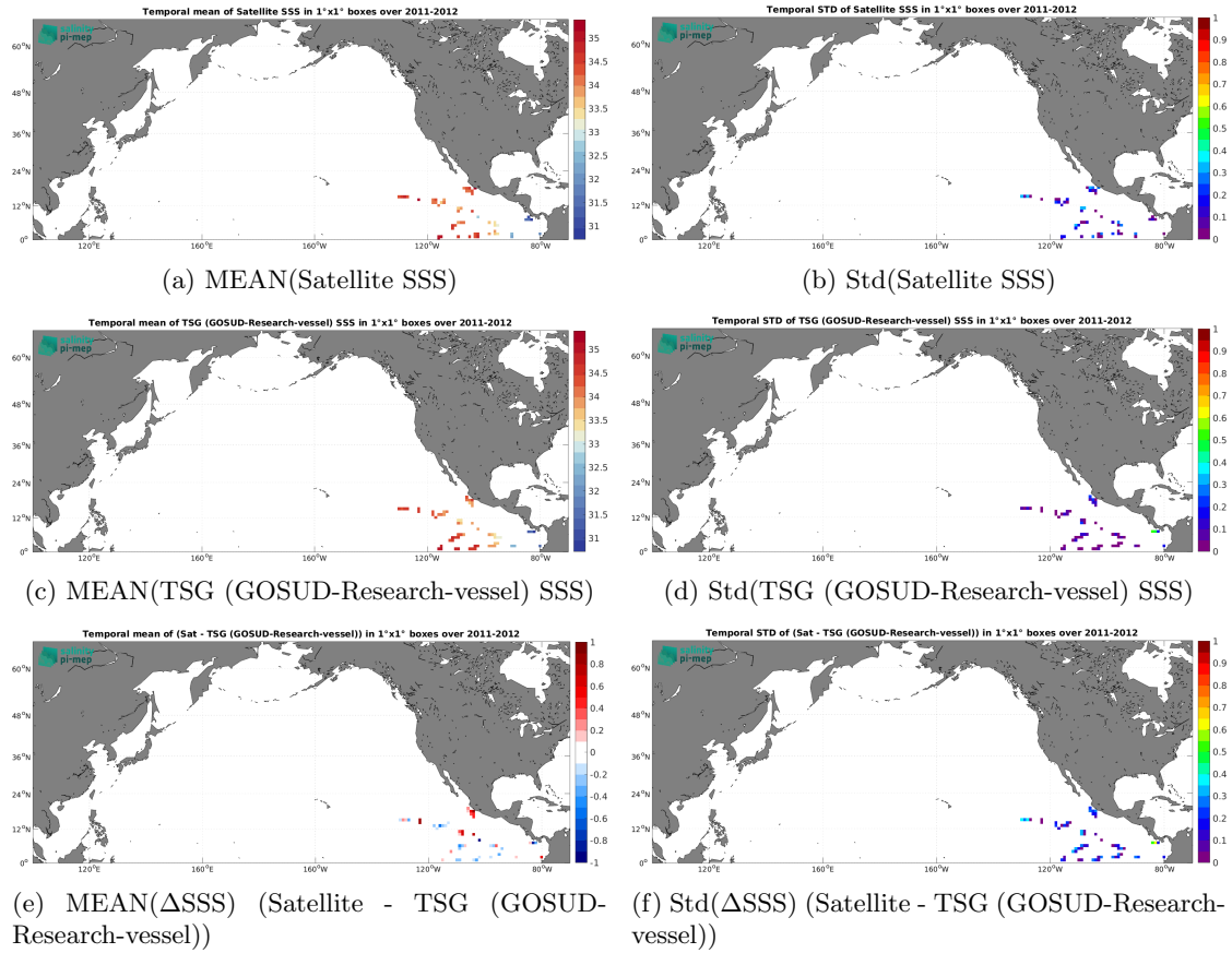
Figure 7: Temporal mean (left) and Std (right) of SSS from Aquarius SSS L2 CAP v5 (JPL) (top), TSG (GOSUD-Research-vessel) (middle), and of \Delta SSS (Satellite - TSG (GOSUD-Research-vessel)). Only match-up pairs are used to generate these maps.
