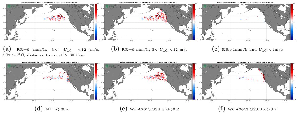
Figure 12: Temporal mean gridded over spatial boxes of size 1^\circ \times 1^\circ of \Delta SSS (Aquarius-L2-JPL-V5 - Sea mammals) for 6 different subdatasets corresponding to:RR=0 mm/h, 3 < U_{10} < 12 m/s, SST >5^\circ C, distance to coast > 800 km (a), RR=0 mm/h, 3 < U_{10} < 12 m/s (b), RR >1 mm/h and U_{10} < 4 m/s (c),MLD <20 m (d),WOA2013 SSS Std <0.2 (e),WOA2013 SSS Std >0.2 (f).
