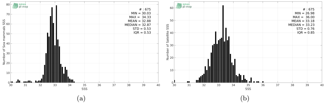
Figure 2: Histograms of SSS from Sea mammals (a) and Aquarius-L2-JPL-V5 (b) considering all match-up pairs per bins of 0.1 over the North Pacific Ocean Pi-MEP region and for the full satellite product period.
