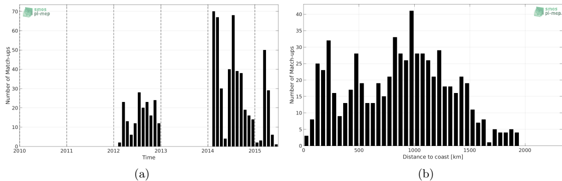
Figure 1: Number of match-ups between Sea mammals and Aquarius-L2-JPL-V5 SSS as a function of time (a) and as function of the distance to coast (b) over the North Pacific Ocean Pi-MEP region and for the full satellite product period.
