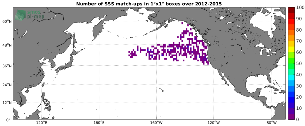
Figure 4: Number of SSS match-ups between Sea mammals SSS and the Aquarius-L2-JPL-V5 SSS product for the North Pacific Ocean Pi-MEP region over 1^\circ \times 1^\circ boxes and for the full satellite product period.
