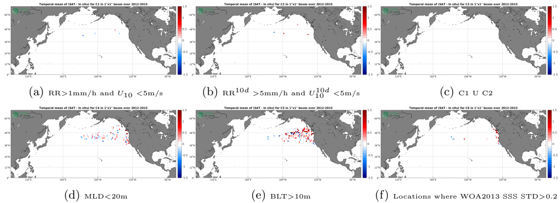
Figure 12: Temporal mean gridded over spatial boxes of size 1^\circ \times 1^\circ of \Delta SSS (Aquarius-L2-JPL-V5 - Sea mammals) for 6 different subdatasets corresponding to: RR > 1\text{mm/h} and U_{10} < 5\text{m/s} (a), RR^{10d} > 5\text{mm/h} and U_{10}^{10d} < 5\text{m/s} (b), C1 U C2 (c), MLD < 20\text{m} (d), BLT > 10\text{m} (e), Locations where WOA2013 SSS STD > 0.2 (f).
