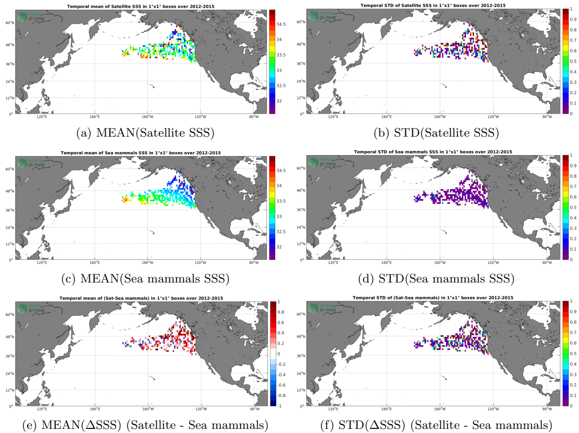
Figure 6: Temporal mean (left) and STD (right) of SSS from Aquarius-L2-JPL-V5 (top), Sea mammals (middle), and of \Delta SSS (Satellite - Sea mammals). Only match-up pairs are used to generate these maps.
