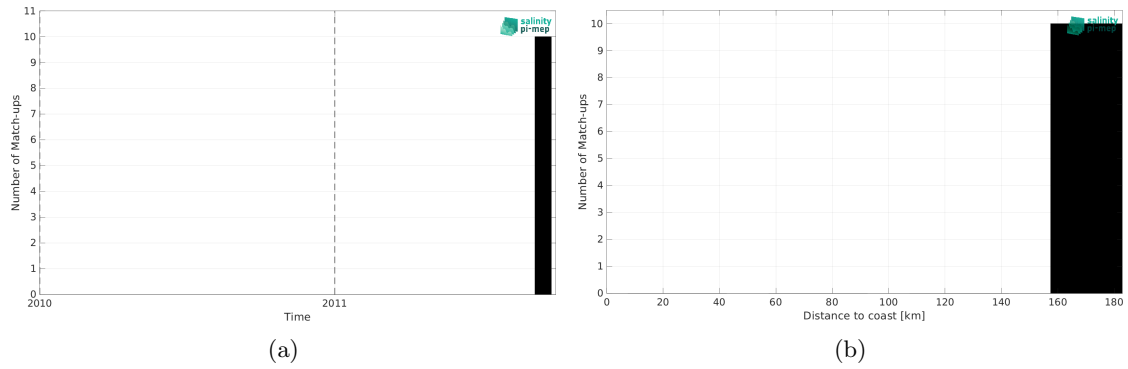
Figure 2: Number of match-ups between Surface drifters and Aquarius SSS L2 CAP v5 (JPL) SSS as a function of time (a) and as function of the distance to coast (b) over the North Pacific Ocean Pi-MEP region and for the full satellite product period.
