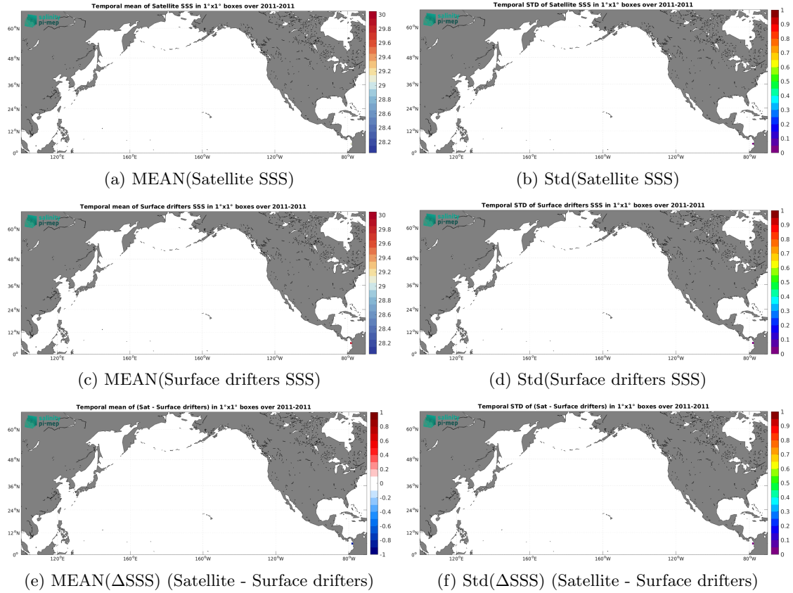
Figure 6: Temporal mean (left) and Std (right) of SSS from Aquarius SSS L2 CAP v5 (JPL) (top), Surface drifters (middle), and of \Delta SSS (Satellite - Surface drifters). Only match-up pairs are used to generate these maps.
