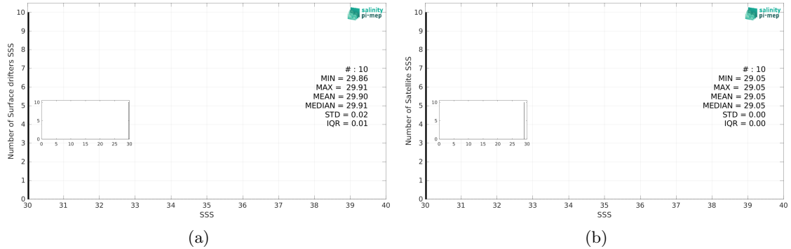
Figure 3: Histograms of SSS from Surface drifters (a) and Aquarius SSS L2 CAP v5 (JPL) (b) considering all match-up pairs per bins of 0.1 over the North Pacific Ocean Pi-MEP region and for the full satellite product period.
