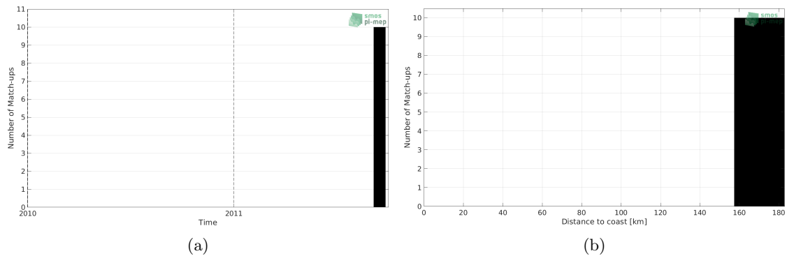
Figure 1: Number of match-ups between Surface drifters and Aquarius SSS L2 CAP v5 (JPL) SSS as a function of time (a) and as function of the distance to coast (b) over the North Pacific Ocean Pi-MEP region and for the full satellite product period.
