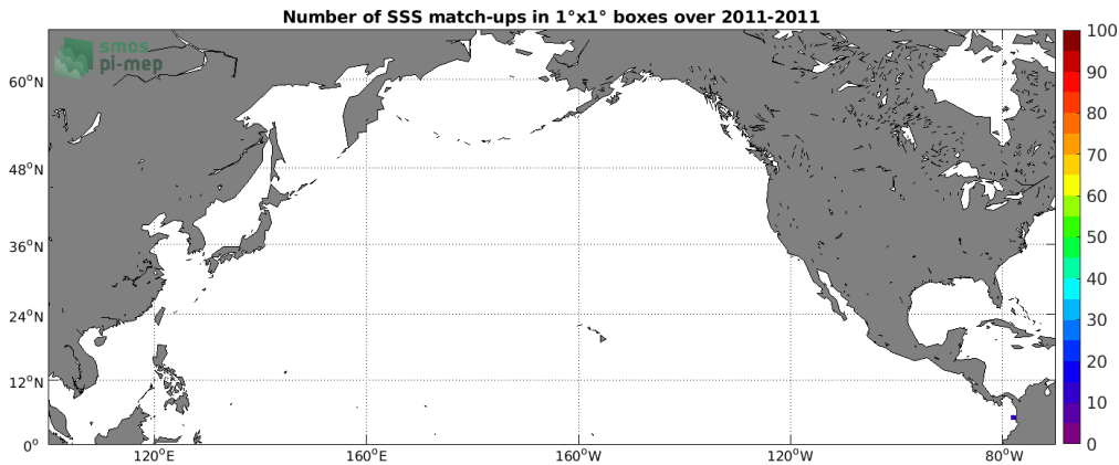
Figure 3: Number of SSS match-ups between Surface drifters SSS and the Aquarius SSS L2 CAP v5 (JPL) SSS product for the North Pacific Ocean Pi-MEP region over 1^\circ \times 1^\circ boxes and for the full satellite product period.
