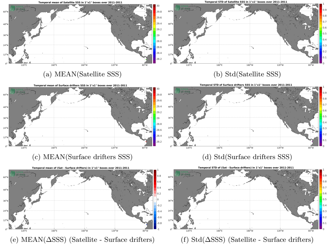
Figure 5: Temporal mean (left) and Std (right) of SSS from Aquarius SSS L2 CAP v5 (JPL) (top), Surface drifters (middle), and of \Delta SSS (Satellite - Surface drifters). Only match-up pairs are used to generate these maps.
