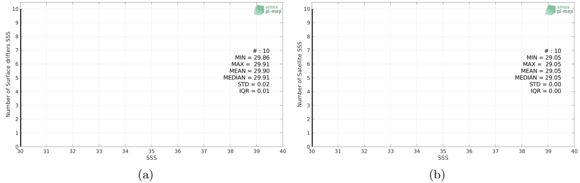
Figure 2: Histograms of SSS from Surface drifters (a) and Aquarius SSS L2 CAP v5 (JPL) (b) considering all match-up pairs per bins of 0.1 over the North Pacific Ocean Pi-MEP region and for the full satellite product period.
