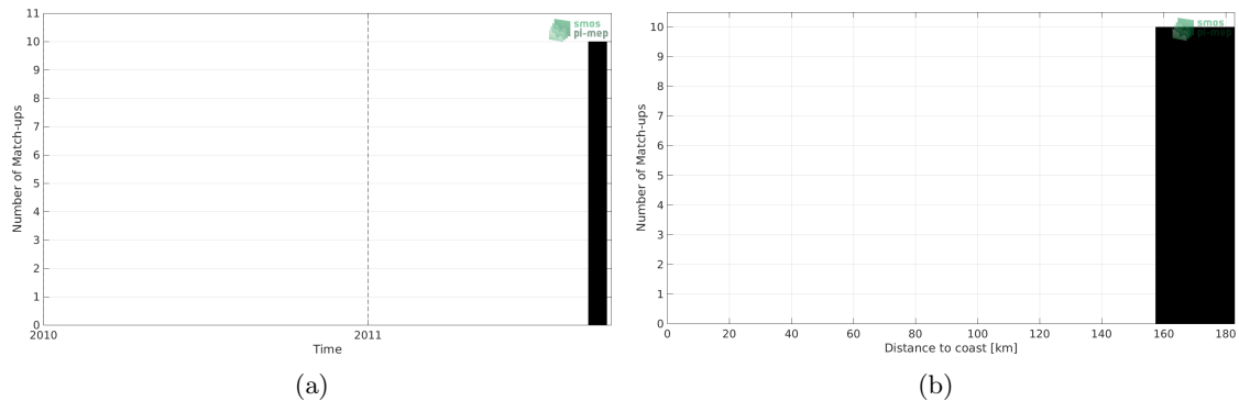
Figure 1: Number of match-ups between Surface drifters and Aquarius SSS L2 CAP v5 (JPL) SSS as a function of time (a) and as function of the distance to coast (b) over the North Pacific Ocean Pi-MEP region and for the full satellite product period.
