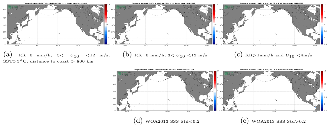
Figure 11: Temporal mean gridded over spatial boxes of size 1^\circ \times 1^\circ of \Delta SSS (Aquarius-L2-JPL-V5 - Surface drifters) for 5 different subdatasets corresponding to:RR=0 mm/h, 3 < U_{10} < 12 m/s, SST >5^\circ C, distance to coast > 800 km (a), RR=0 mm/h, 3 < U_{10} < 12 m/s (b), RR >1 mm/h and U_{10} < 4 m/s (c), WOA2013 SSS Std <0.2 (d), WOA2013 SSS Std >0.2 (e).
