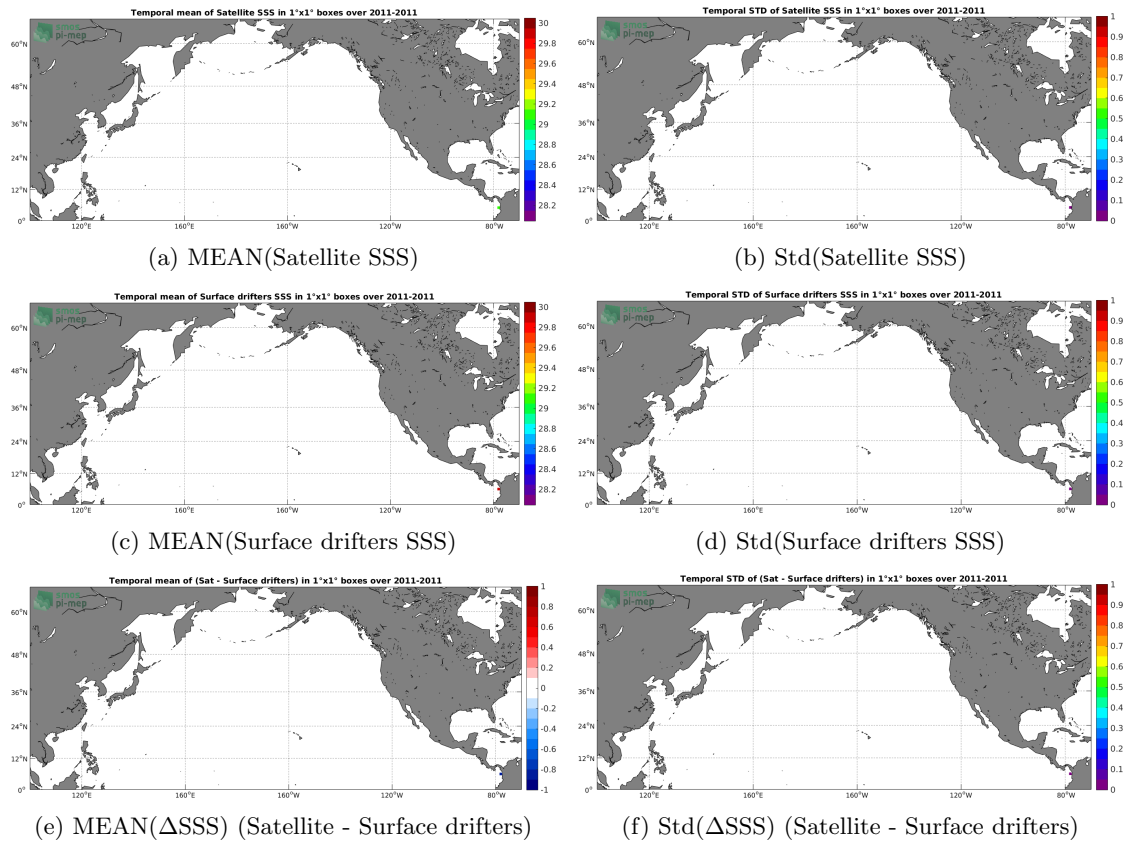
Figure 5: Temporal mean (left) and Std (right) of SSS from Aquarius-L2-JPL-V5 (top), Surface drifters (middle), and of \Delta SSS (Satellite - Surface drifters). Only match-up pairs are used to generate these maps.
