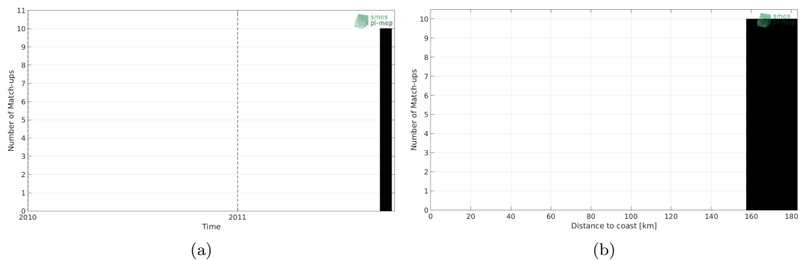
Figure 1: Number of match-ups between Surface drifters and Aquarius-L2-JPL-V5 SSS as a function of time (a) and as function of the distance to coast (b) over the North Pacific Ocean Pi-MEP region and for the full satellite product period.
