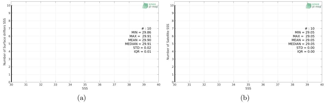
Figure 2: Histograms of SSS from Surface drifters (a) and Aquarius-L2-JPL-V5 (b) considering all match-up pairs per bins of 0.1 over the North Pacific Ocean Pi-MEP region and for the full satellite product period.
