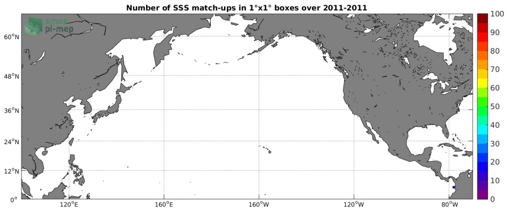
Figure 3: Number of SSS match-ups between Surface drifters SSS and the Aquarius-L2-JPL-V5 SSS product for the North Pacific Ocean Pi-MEP region over 1°x1° boxes and for the full satellite product period.
