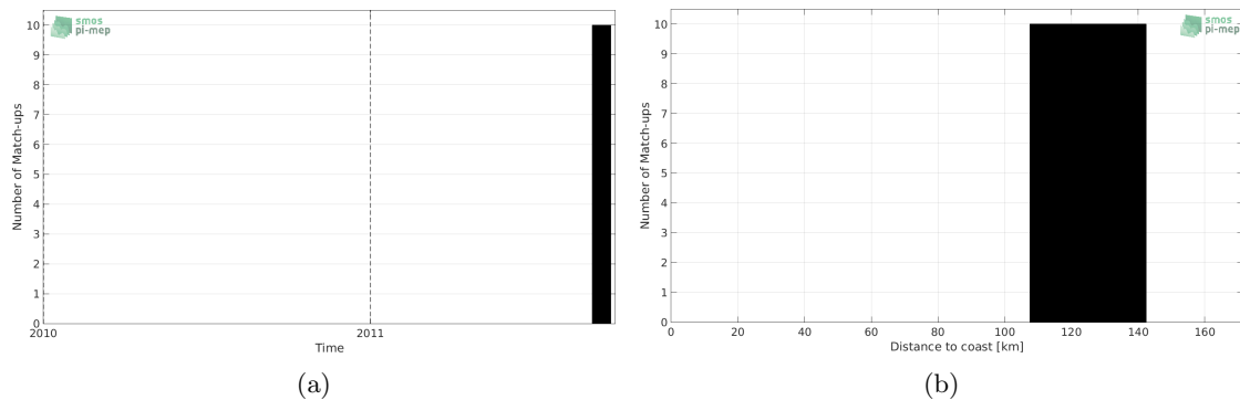
Figure 1: Number of match-ups between Surface drifters and Aquarius-L2-JPL-V5 SSS as a function of time (a) and as function of the distance to coast (b) over the North Pacific Ocean Pi-MEP region and for the full satellite product period.
