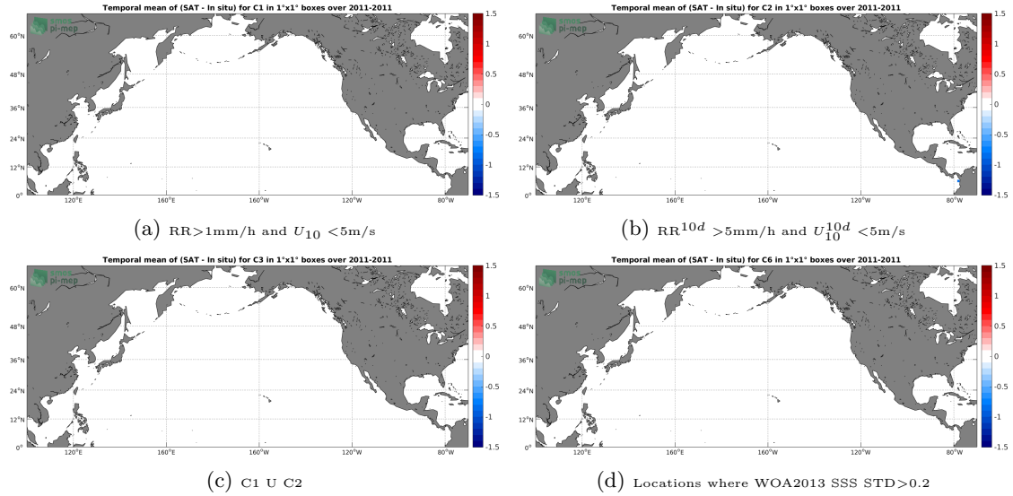
Figure 11: Temporal mean gridded over spatial boxes of size 1^\circ \times 1^\circ of \Delta SSS (Aquarius-L2-JPL-V5 - Surface drifters) for 4 different subdatasets corresponding to: RR > 1mm/h and U_{10} < 5\text{m/s} (a), RR^{10d} > 5\text{mm/h} and U_{10}^{10d} < 5\text{m/s} (b), C1 U C2 (c), Locations where WOA2013 SSS STD > 0.2 (d).
