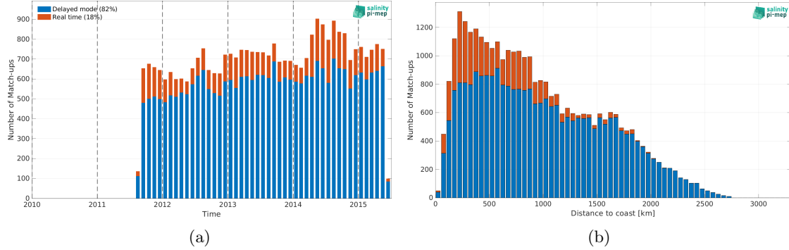
Figure 2: Number of match-ups between Argo and Aquarius SSS L2 CAP v5 (JPL) SSS as a function of time (a) and as function of the distance to coast (b) over the North Pacific Ocean Pi-MEP region and for the full satellite product period.
