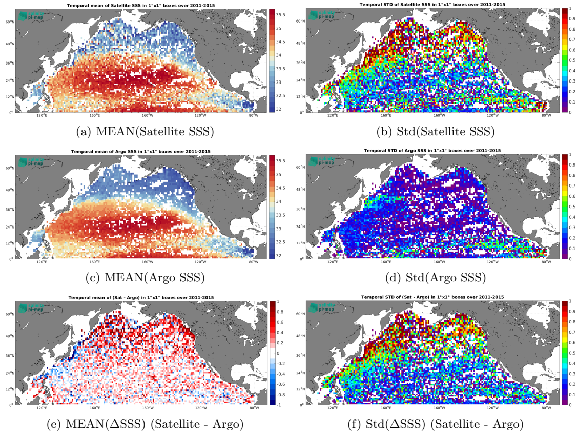
Figure 7: Temporal mean (left) and Std (right) of SSS from Aquarius SSS L2 CAP v5 (JPL) (top), Argo (middle), and of \Delta SSS (Satellite - Argo). Only match-up pairs are used to generate these maps.
