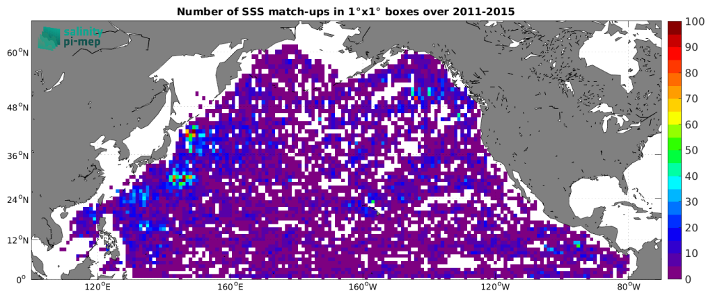
Figure 5: Number of SSS match-ups between Argo SSS and the Aquarius SSS L2 CAP v5 (JPL) SSS product for the North Pacific Ocean Pi-MEP region over 1^\circ \times 1^\circ boxes and for the full satellite product period.
