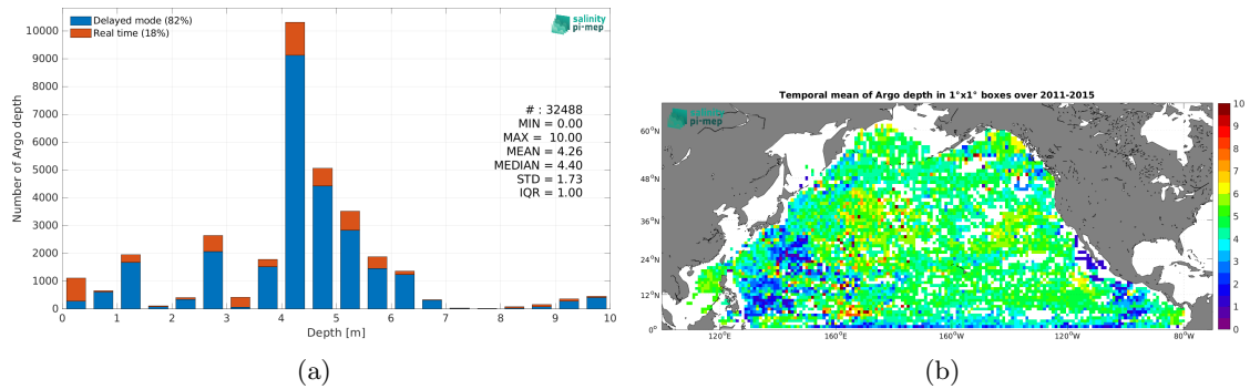
Figure 4: Histograms of the depth of the upper level SSS measurements from Argo in the Match-up DataBase for the North Pacific Ocean Pi-MEP region (a) and temporal mean spatial distribution of pressure of the in situ SSS data over 1^\circ \times 1^\circ boxes and for the full satellite product period (b).
