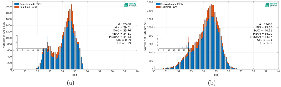
Figure 3: Histograms of SSS from Argo (a) and Aquarius SSS L2 CAP v5 (JPL) (b) considering all match-up pairs per bins of 0.1 over the North Pacific Ocean Pi-MEP region and for the full satellite product period.
