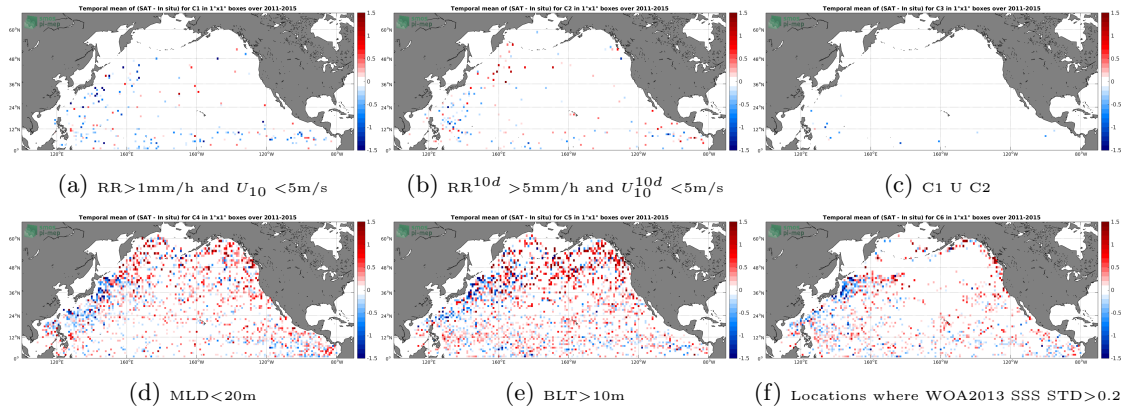
Figure 12: Temporal mean gridded over spatial boxes of size 1°x1° of \Delta SSS (Aquarius-L2-JPL-V5 - Argo) for 6 different subdatasets corresponding to:RR>1mm/h and U_{10} < 5m/s (a), RR^{10d} > 5mm/h and U_{10}^{10d} < 5m/s (b), C1 U C2 (c),MLD<20m (d),BLT>10m (e),Locations where WOA2013 SSS STD>0.2 (f).
