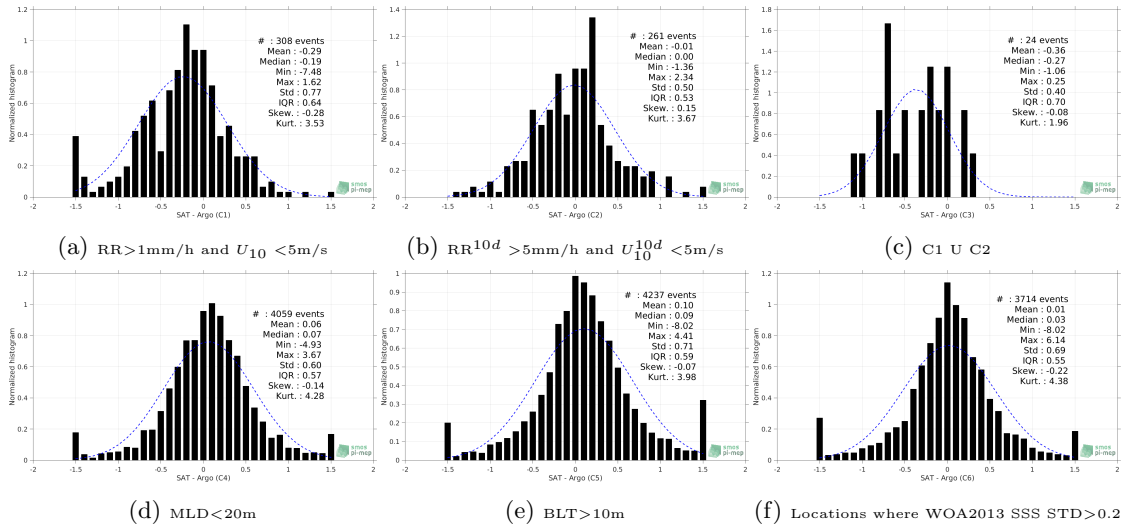
Figure 13: Normalized histogram of \Delta SSS (Aquarius-L2-JPL-V5 - Argo) for 6 different subdatasets corresponding to: RR>1mm/h and U_{10} < 5m/s (a), RR^{10d} > 5mm/h and U_{10}^{10d} < 5m/s (b), C1 U C2 (c),MLD<20m (d),BLT>10m (e),Locations where WOA2013 SSS STD>0.2 (f).
