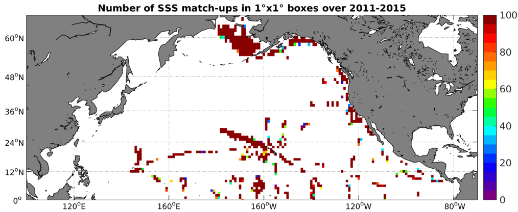
Figure 4: Number of SSS match-ups between TSG-SAMOS SSS and the AQUARIUS-L2-JPL-V4 SSS product for the North Pacific Ocean Pi-MEP region over 1^\circ \times 1^\circ boxes and for the full satellite product period.
