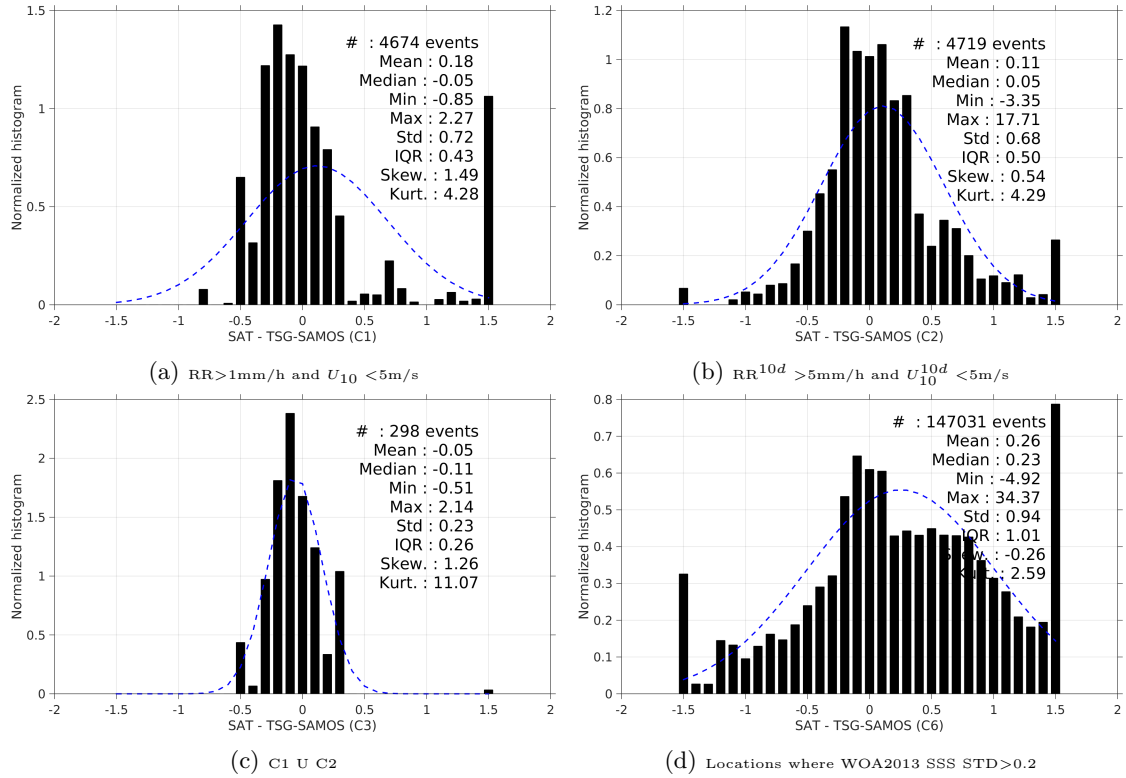
Figure 13: Normalized histogram of \Delta\text{SSS} (AQUARIUS-L2-JPL-V4 - TSG-SAMOS) for 6 different subdatasets corresponding to: \text{RR} > 1\text{mm/h} and U_{10} < 5\text{m/s} (a), \text{RR}^{10d} > 5\text{mm/h} and U_{10}^{10d} < 5\text{m/s} (b), C1 \cup C2 (c), Locations where WOA2013 SSS STD > 0.2 (d).
