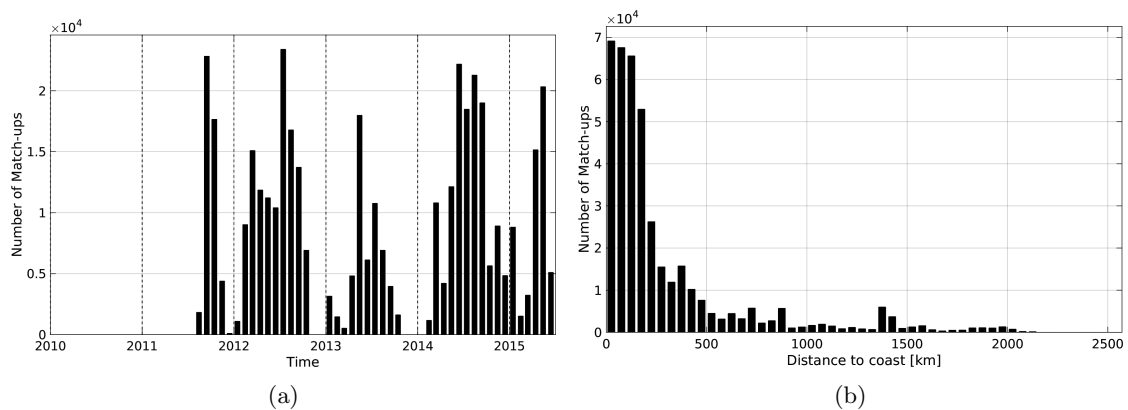
Figure 1: Number of match-ups between TSG-SAMOS and AQUARIUS-L2-JPL-V4 SSS as a function of time (a) and as function of the distance to coast (b) over the North Pacific Ocean Pi-MEP region and for the full satellite product period.
