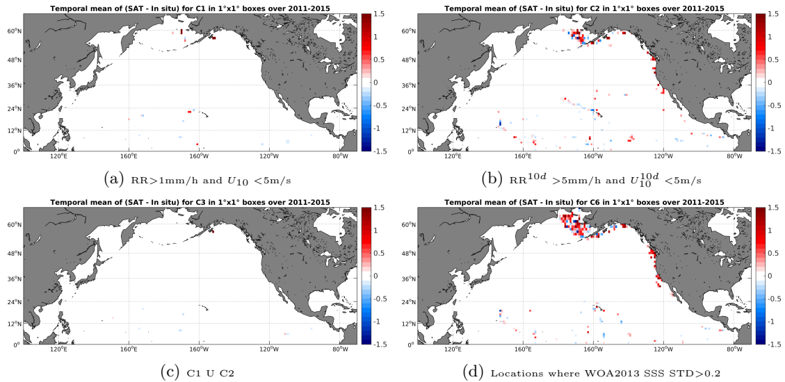
Figure 12: Temporal mean gridded over spatial boxes of size 1^\circ \times 1^\circ of \Delta SSS (AQUARIUS-L2-JPL-V4 - TSG-SAMOS) for 4 different subdatasets corresponding to: RR > 1\text{mm/h} and U_{10} < 5\text{m/s} (a), RR^{10d} > 5\text{mm/h} and U_{10}^{10d} < 5\text{m/s} (b), C1 U C2 (c), Locations where WOA2013 SSS STD > 0.2 (d).
