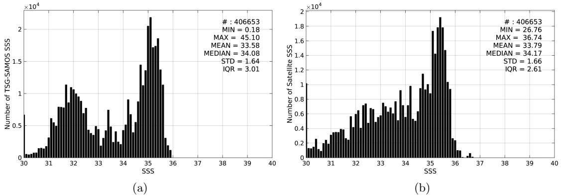
Figure 2: Histograms of SSS from TSG-SAMOS (a) and AQUARIUS-L2-JPL-V4 (b) considering all match-up pairs per bins of 0.1 over the North Pacific Ocean Pi-MEP region and for the full satellite product period.
