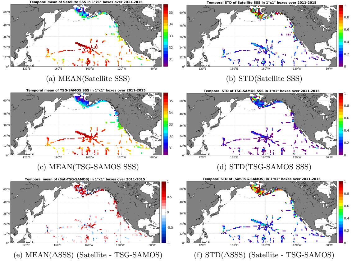
Figure 6: Temporal mean (left) and STD (right) of SSS from AQUARIUS-L2-JPL-V4 (top), TSG-SAMOS (middle), and of \Delta SSS (Satellite - TSG-SAMOS). Only match-up pairs are used to generate these maps.
