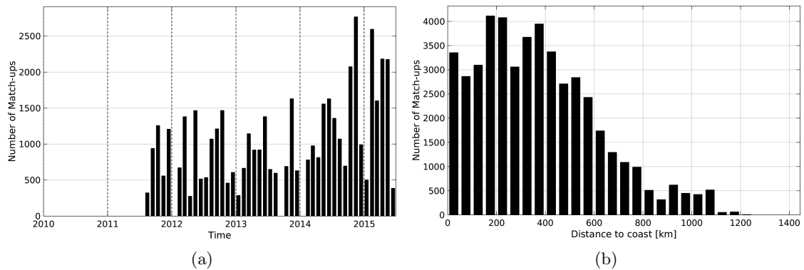
Figure 1: Number of match-ups between TSG-LEGOS-DM and AQUARIUS-L2-JPL-V4 SSS as a function of time (a) and as function of the distance to coast (b) over the North Pacific Ocean Pi-MEP region and for the full satellite product period.
