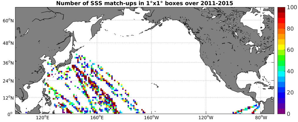
Figure 4: Number of SSS match-ups between TSG-LEGOS-DM SSS and the AQUARIUS-L2-JPL-V4 SSS product for the North Pacific Ocean Pi-MEP region over 1^\circ \times 1^\circ boxes and for the full satellite product period.
