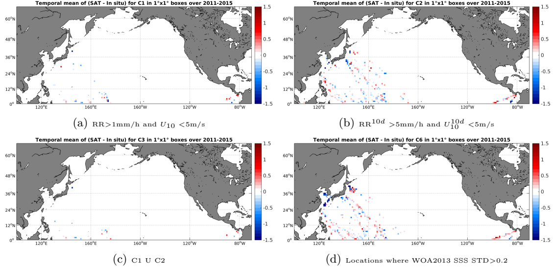
Figure 12: Temporal mean gridded over spatial boxes of size 1^\circ \times 1^\circ of \Delta SSS (AQUARIUS-L2-JPL-V4 - TSG-LEGOS-DM) for 4 different subdatasets corresponding to: RR > 1 mm/h and U_{10} < 5 m/s (a), RR^{10d} > 5 mm/h and U_{10}^{10d} < 5 m/s (b), C1 U C2 (c), Locations where WOA2013 SSS STD > 0.2 (d).
