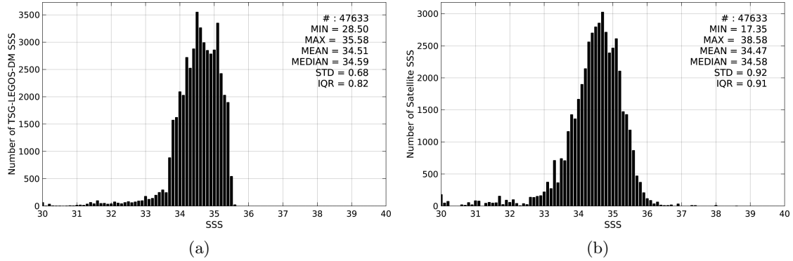
Figure 2: Histograms of SSS from TSG-LEGOS-DM (a) and AQUARIUS-L2-JPL-V4 (b) considering all match-up pairs per bins of 0.1 over the North Pacific Ocean Pi-MEP region and for the full satellite product period.
