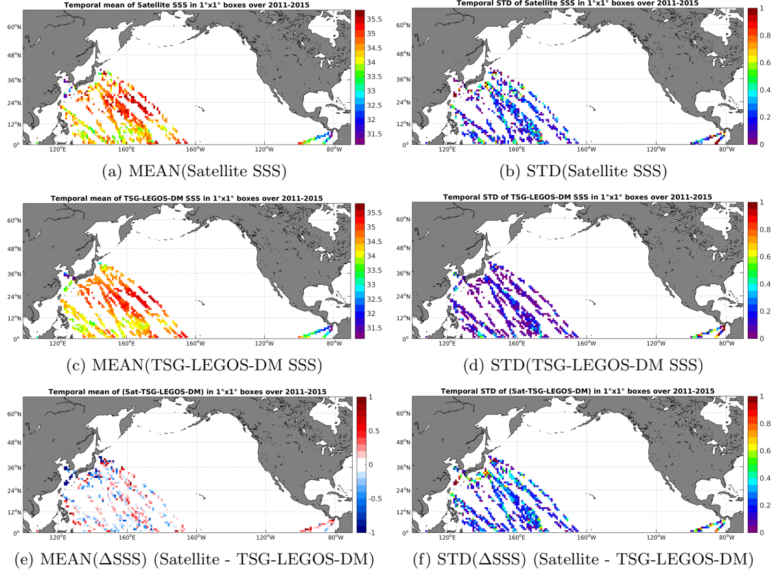
Figure 6: Temporal mean (left) and STD (right) of SSS from AQUARIUS-L2-JPL-V4 (top), TSG-LEGOS-DM (middle), and of \Delta SSS (Satellite - TSG-LEGOS-DM). Only match-up pairs are used to generate these maps.
