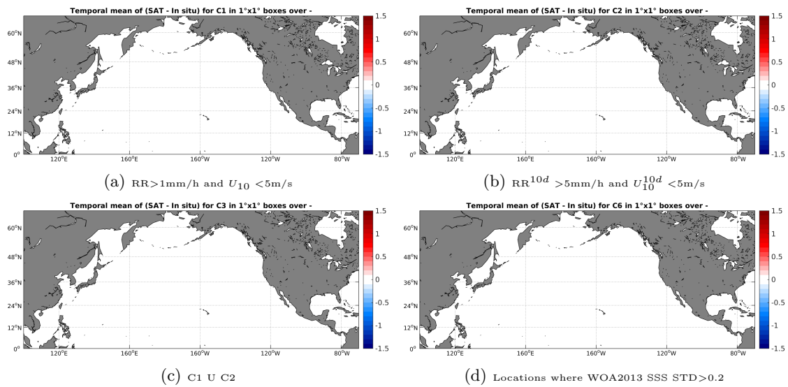
Figure 12: Temporal mean gridded over spatial boxes of size 1^\circ \times 1^\circ of \Delta SSS (AQUARIUS-L2-JPL-V4 - TSG-GOSUD-Sailing-ship) for 4 different subdatasets corresponding to:RR >1 mm/h and U_{10} < 5 m/s (a), RR ^{10d} > 5 mm/h and U_{10}^{10d} < 5 m/s (b), C1 U C2 (c),Locations where WOA2013 SSS STD >0.2 (d).
