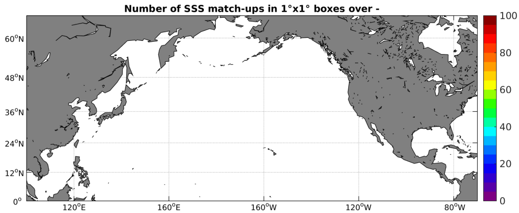
Figure 4: Number of SSS match-ups between TSG-GOSUD-Sailing-ship SSS and the AQUARIUS-L2-JPL-V4 SSS product for the North Pacific Ocean Pi-MEP region over 1^\circ \times 1^\circ boxes and for the full satellite product period.
